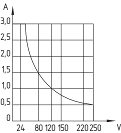
Switching capacity
