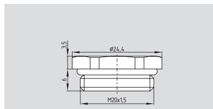
EX-certified screw plug
