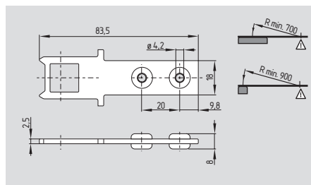
AZ 335/355-B1-2245 with rubber mounting
