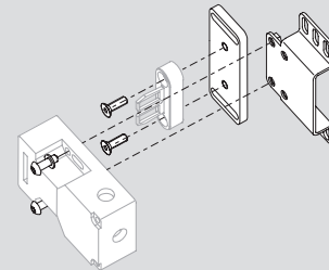
Mounting set MS AZ 15/16
