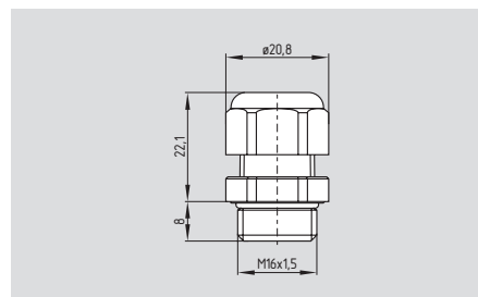
EX-certified screwed cable gland
