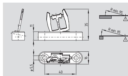
Shortened angled actuator B6S
