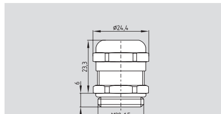
EX-certified screwed cable gland
