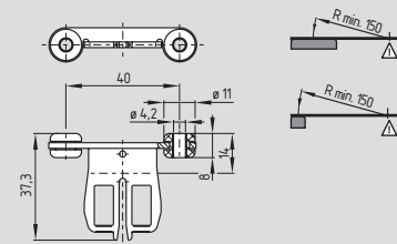
AZ 15/16-B1-2245 with rubber mounting
