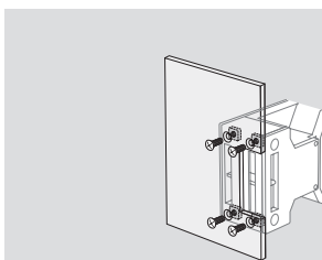
Front mounting AZ 15/16 -1762
