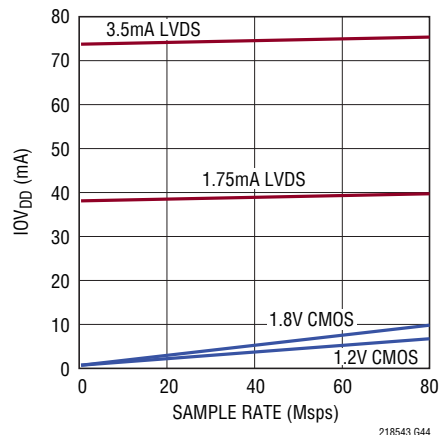
LTC2183: I_{O_VDD} vs Sample Rate, 5\text{MHz} , -1\text{dBFS} Sine Wave Input on Each Channel
