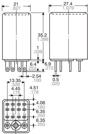
External dimensions
