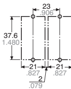
Chassis (Panel) cutout in tandem mounting
