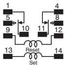
Schematic (Bottom view)
