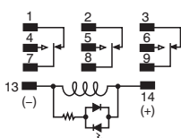
LED DC type
