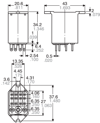
External dimensions
