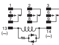
LED AC type
