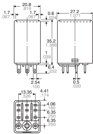
External dimensions
