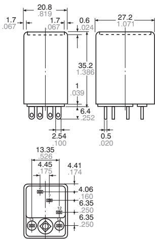
External dimensions
