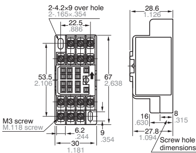
External dimensions
