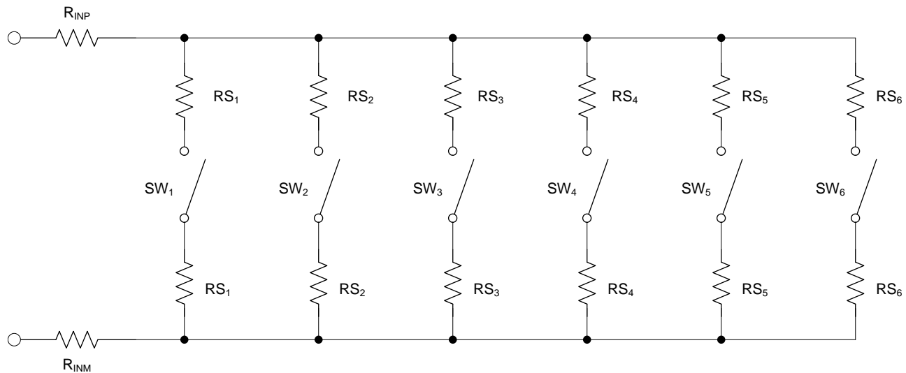
Figure 21. Programmable Attenuator
