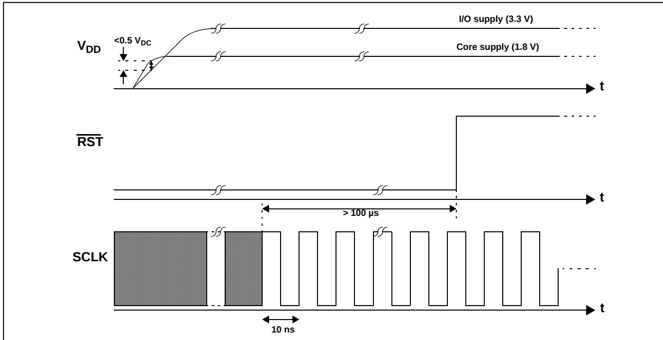
Figure 17 - Powering Up the ZL30302
