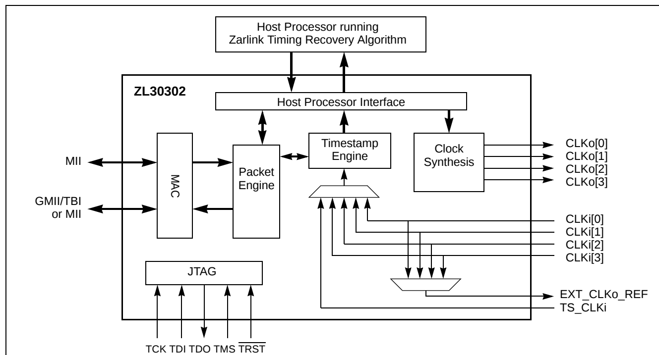
Figure 1 - ZL30302 Functional Block Diagram
