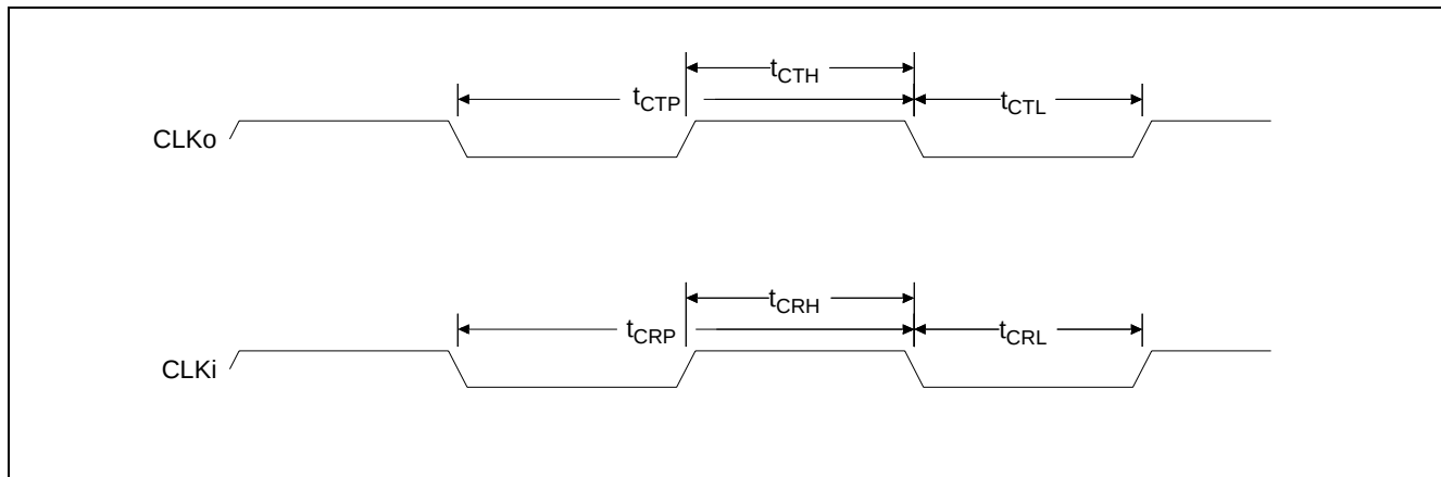
Figure 18 - Clock Interface Timing
