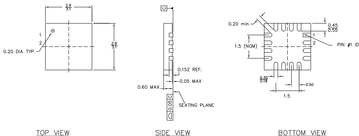
Figure 18. 16-pin Chip On Lead (3 × 3 × 0.6 mm) LG16A/LD16A (Sawn) Package Outline, 001-09116
