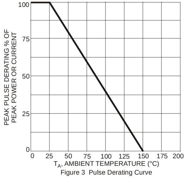
Figure 3 Pulse Derating Curve
