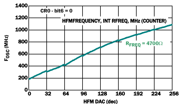
FIGURE 6. HFM CONTROL; V_{SO} = 5.0V
