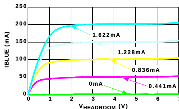
FIGURE 4. I_{BLUE} READ vs V_{HEADROOM} vs I_{AP} , (REG 1-21 = 88h) ( V_{SO} = 5.0V ), ( R_{SET} = 620\Omega )
