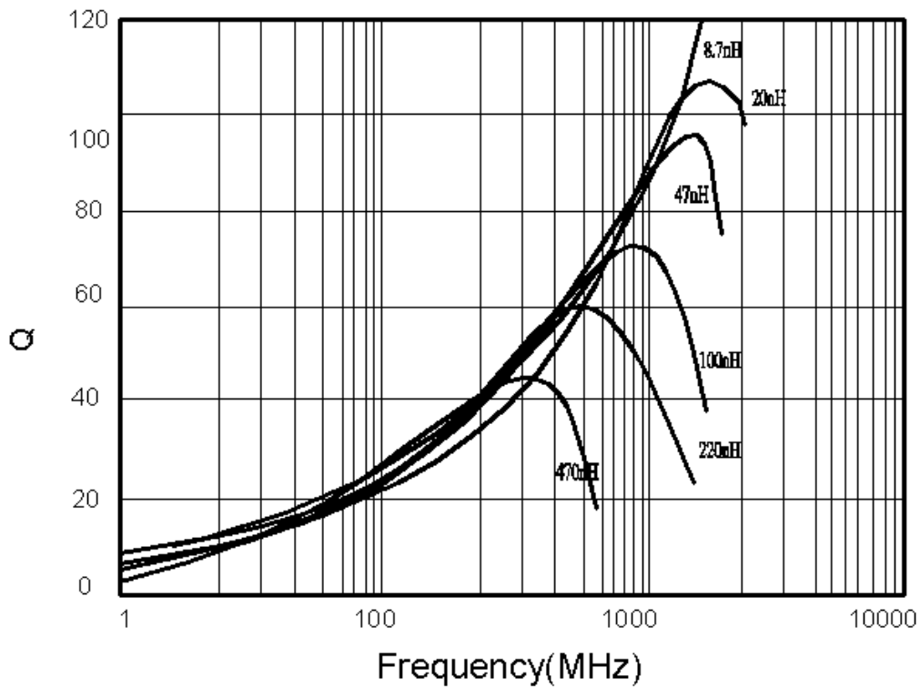
TYPICAL Q vs FREQUENCY
