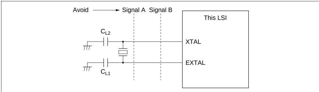
Figure 24.4 Example of Incorrect Board Design
