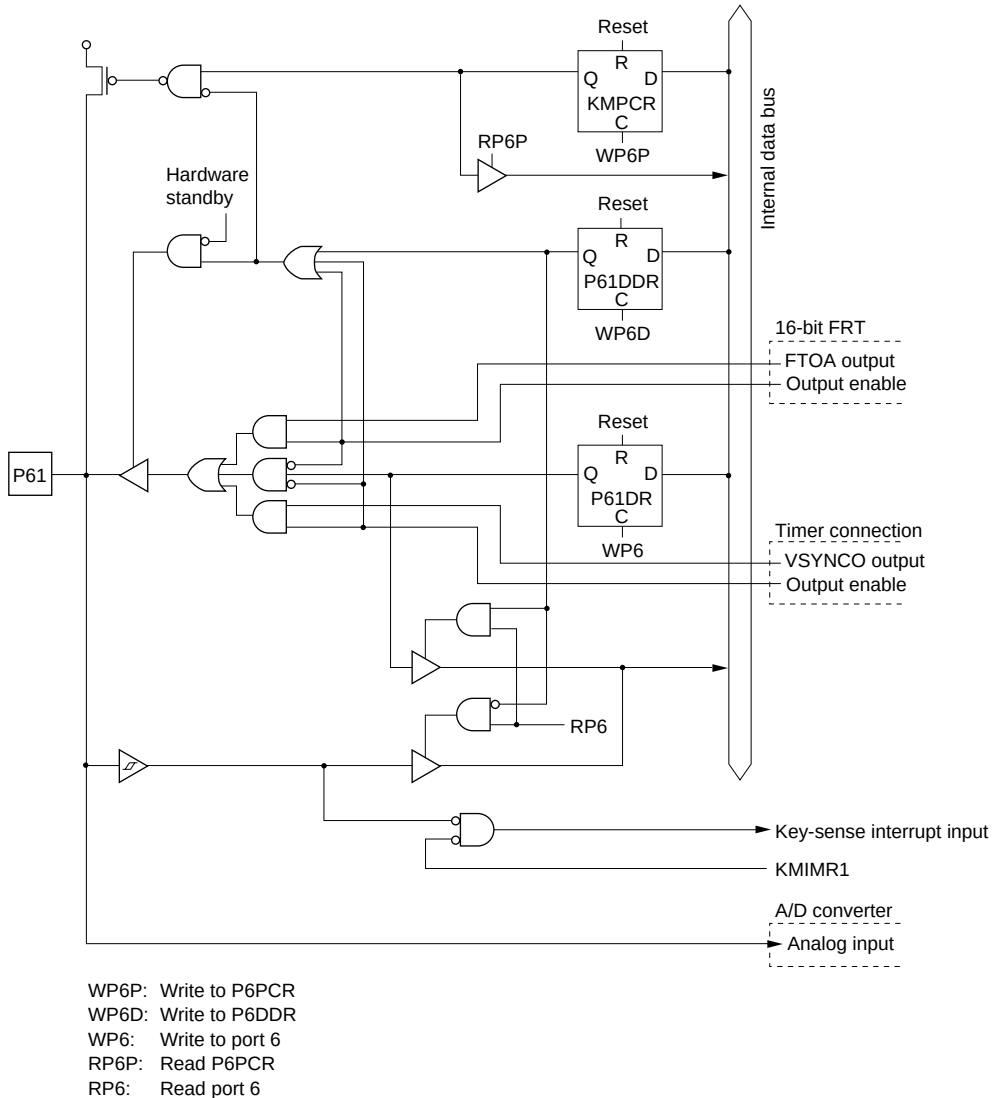
Figure C.17 Port 6 Block Diagram (Pin P61)
