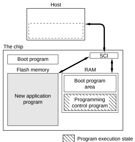
Figure 23.4 Boot Mode
