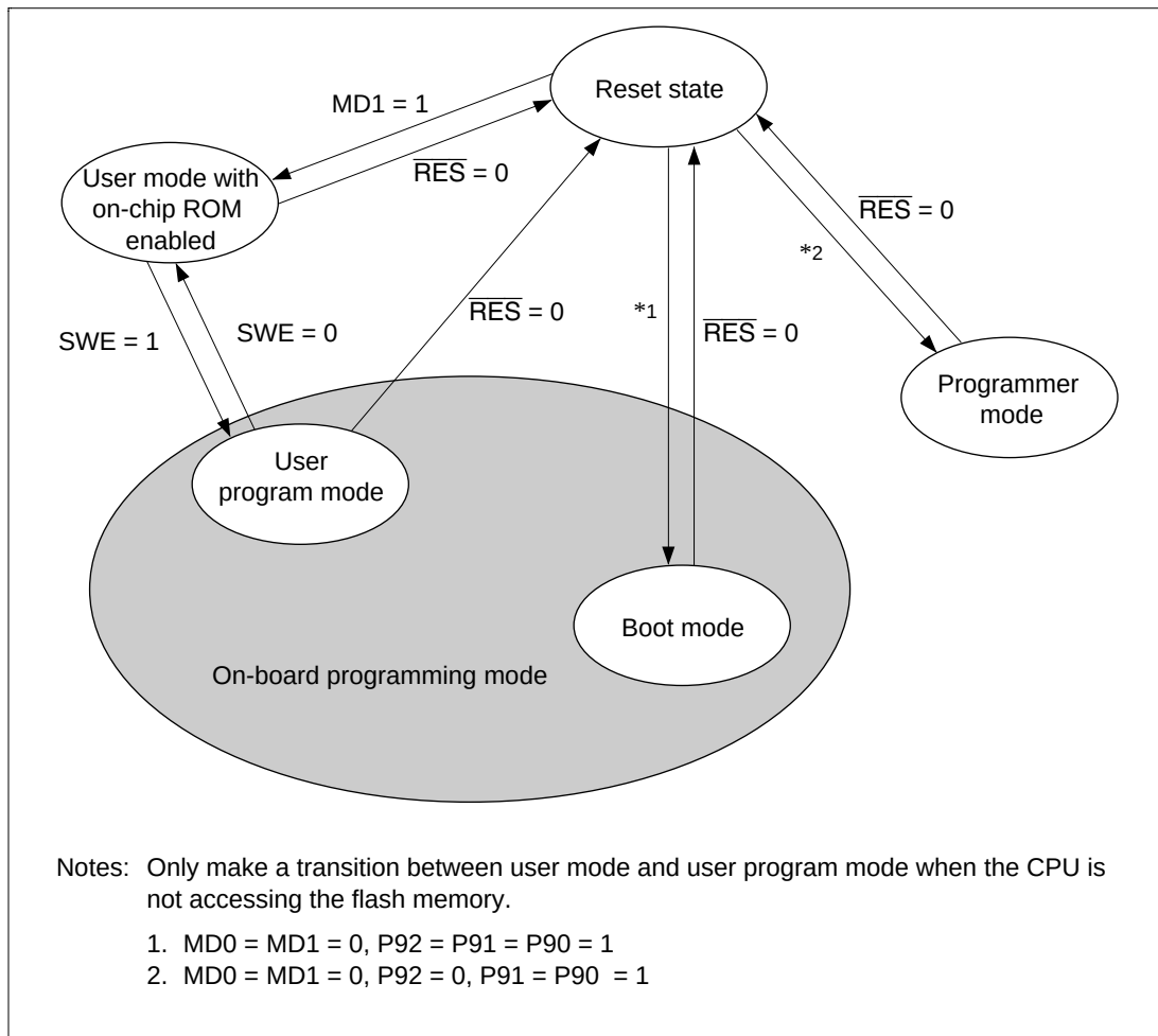
Figure 23.3 Flash Memory Mode Transitions
