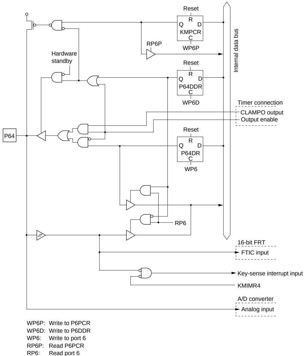
Figure C.18 Port 6 Block Diagram (Pin P64)
