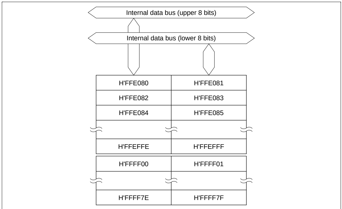
Figure 21.1 Block Diagram of RAM (H8S/2148, H8S/2144, H8S/2143)
