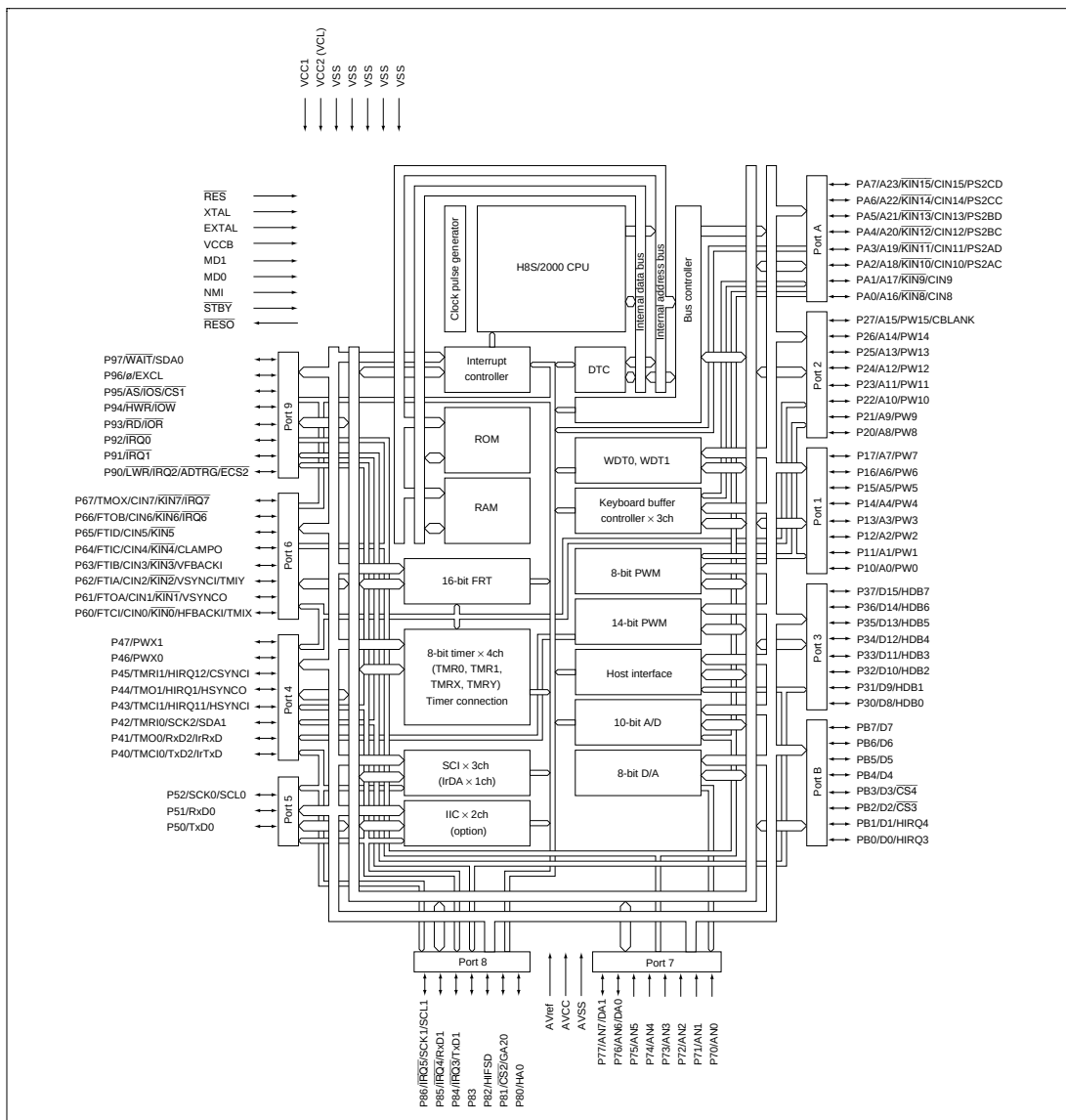
Figure 1.1 (a) Internal Block Diagram of H8S/2148 Series
