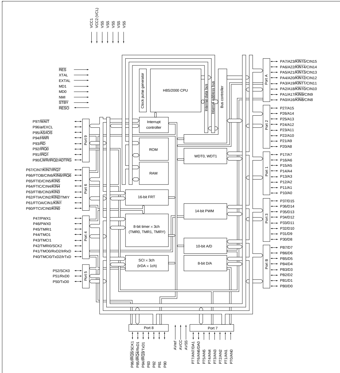
Figure 1.1 (c) Internal Block Diagram of H8S/2144 Series
