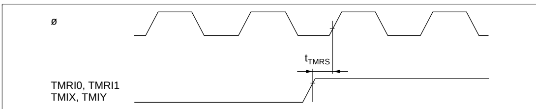
Figure 26.20 8-Bit Timer Reset Input Timing
