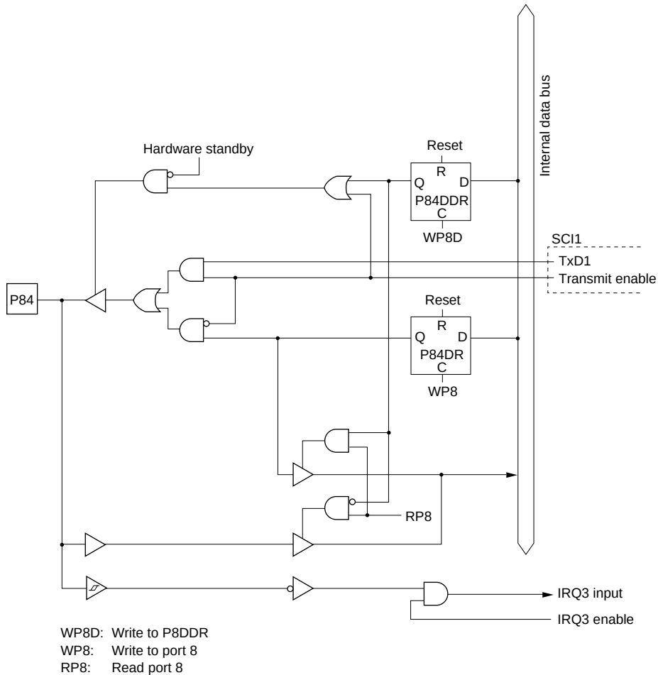
Figure C.26 Port 8 Block Diagram (Pin P84)
