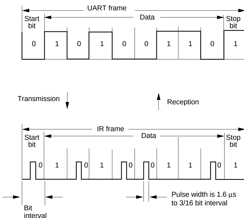
Figure 15.22 IrDA Transmit/Receive Operations
