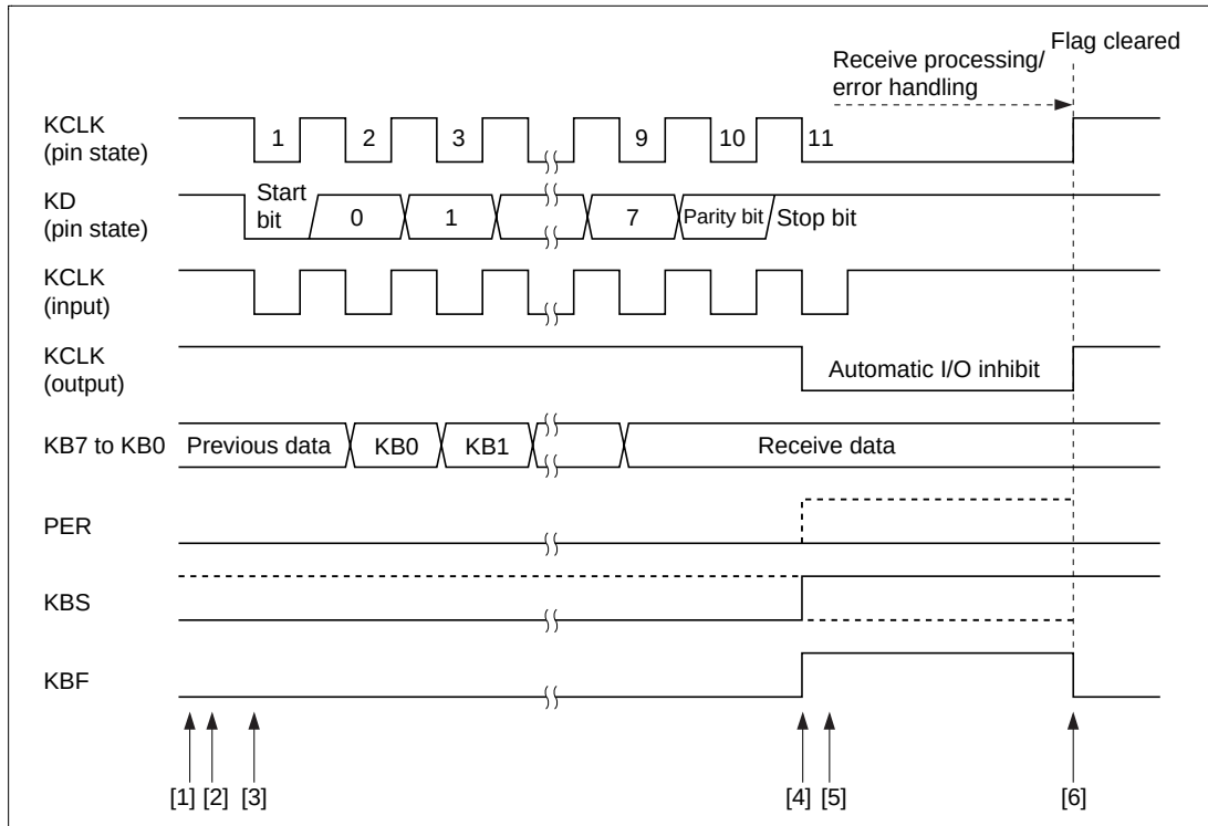
Figure 17.4 Receive Timing
