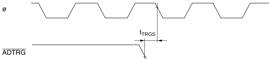
Figure 26.24 A/D Converter External Trigger Input Timing
