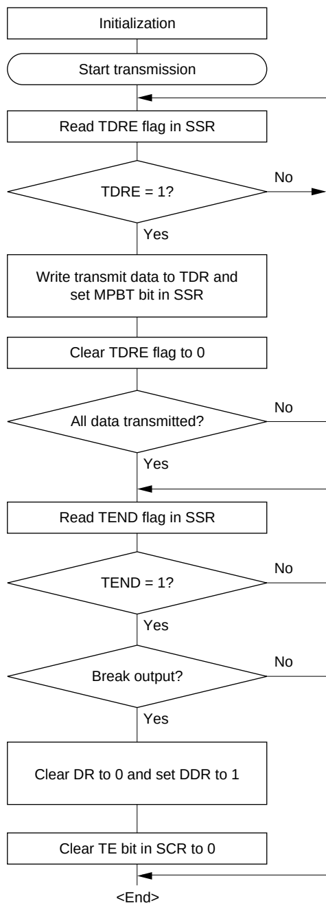
Figure 15.10 Sample Multiprocessor Serial Transmission Flowchart
