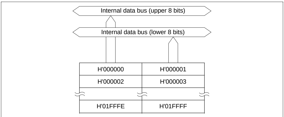
Figure 23.1 ROM Block Diagram (A-mask versions of the H8S/2148 F-ZTAT and H8S/2144 F-ZTAT)
