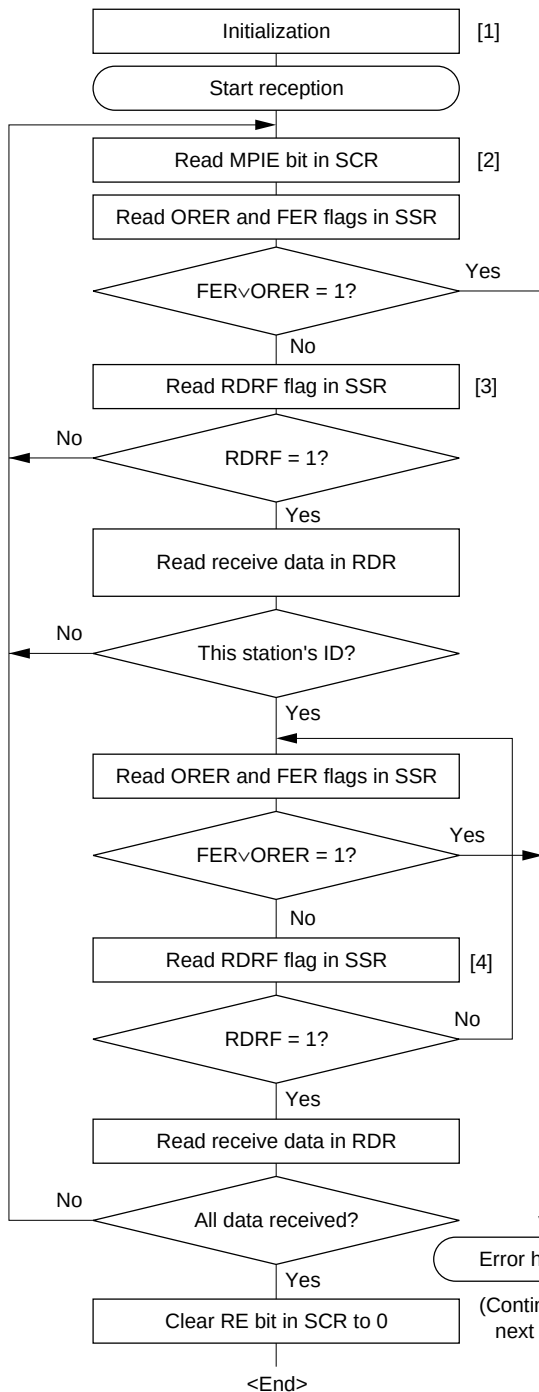
Figure 15.12 Sample Multiprocessor Serial Reception Flowchart
