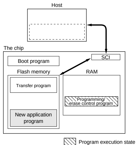
Figure 22.5 User Program Mode (Example)
