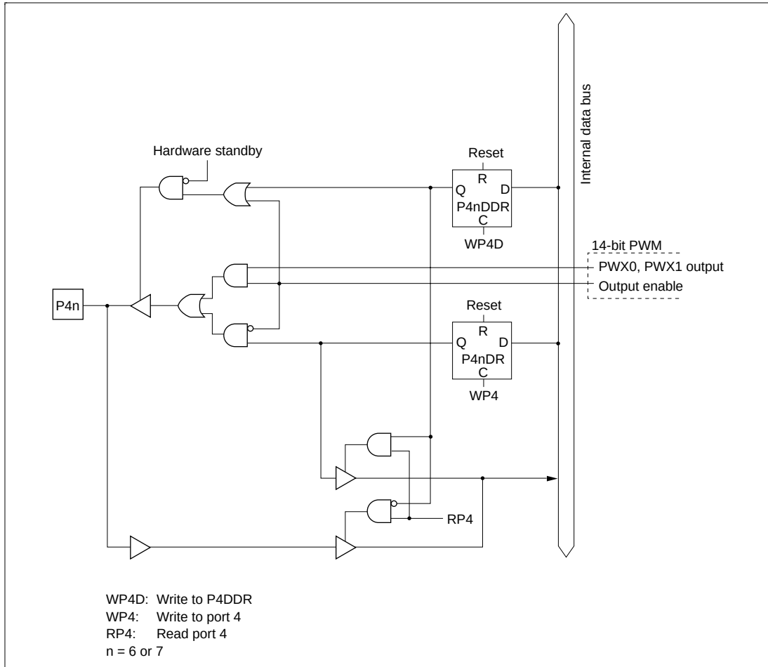
Figure C.12 Port 4 Block Diagram (Pins P46, P47)
