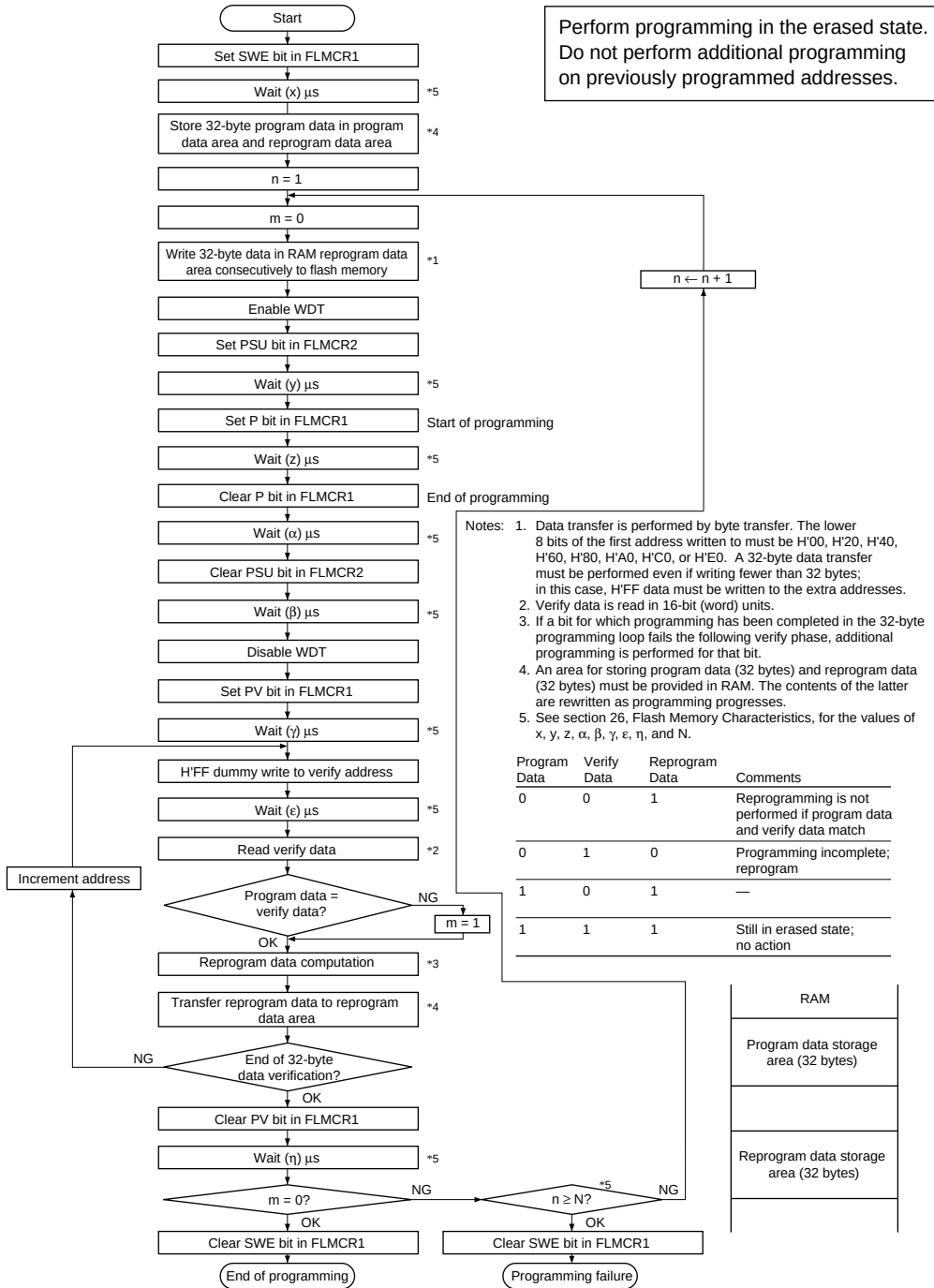
Figure 22.12 Program/Program-Verify Flowchart
