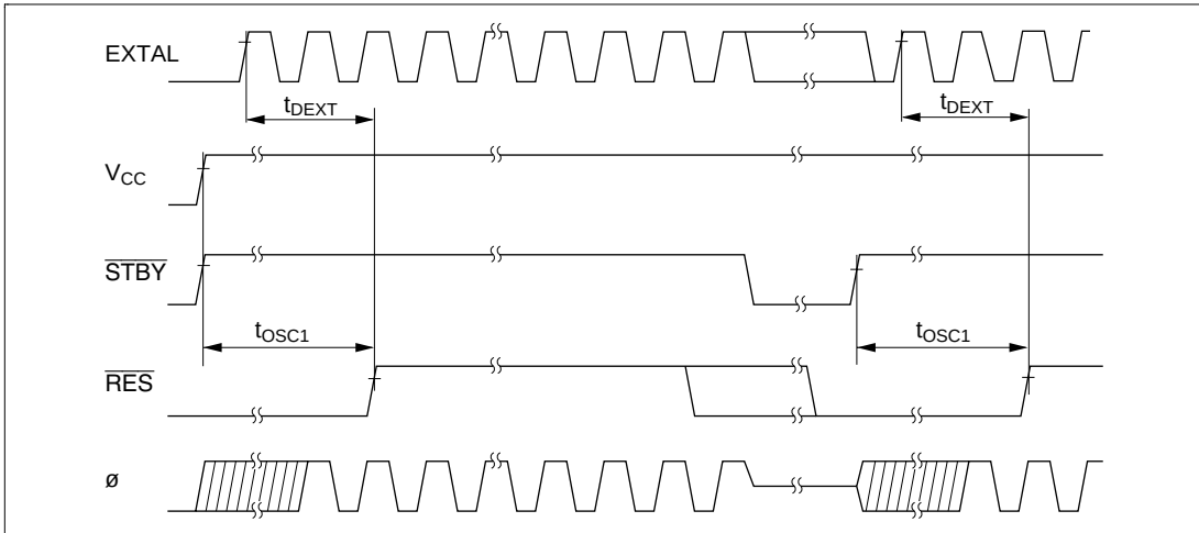
Figure 26.6 Oscillation Settling Timing
