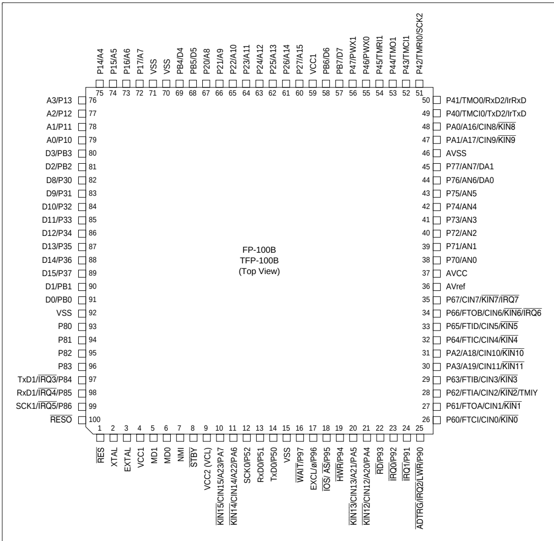
Figure 1.2 (c) Pin Arrangement of H8S/2144 Series (FP-100B, TFP-100B: Top View)
