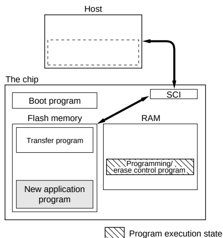
Figure 23.5 User Program Mode (Example)
