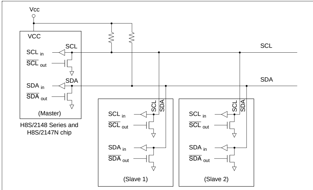
Figure 16.2 I²C Bus Interface Connections (Example: H8S/2148 Series and H8S/2147N Chip as Master)
