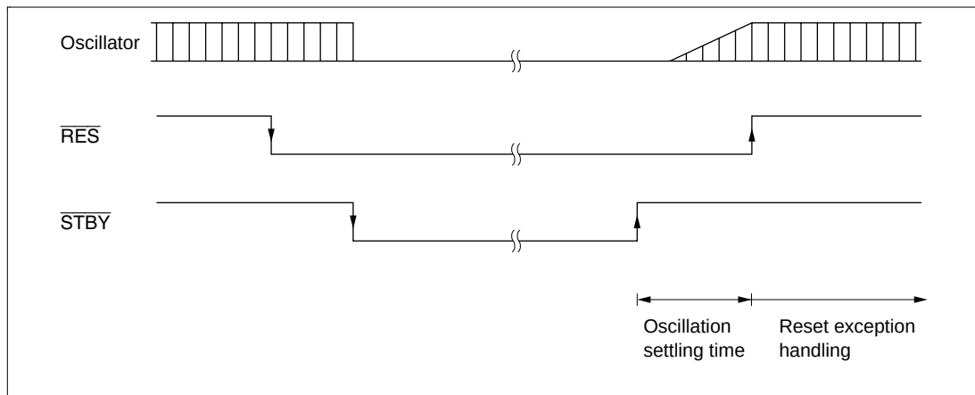
Figure 25.4 Hardware Standby Mode Timing
