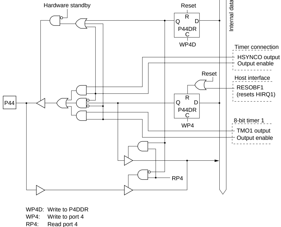
Figure C.10 Port 4 Block Diagram (Pin P44)
