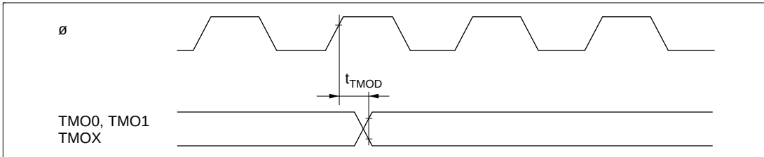
Figure 26.18 8-Bit Timer Output Timing
