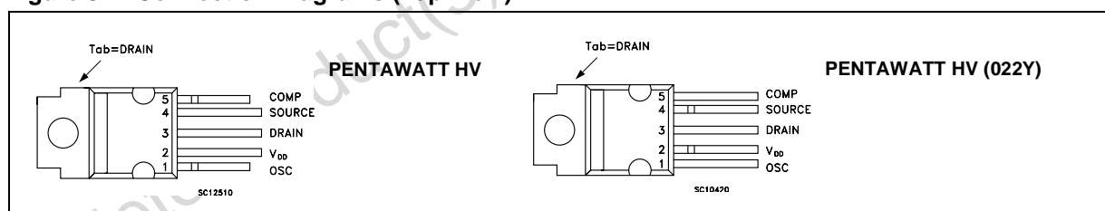
Figure 3. Connection Diagrams (Top View)
