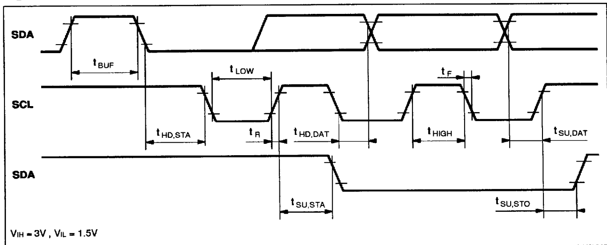
Figure 2 : Serial Bus Timing
