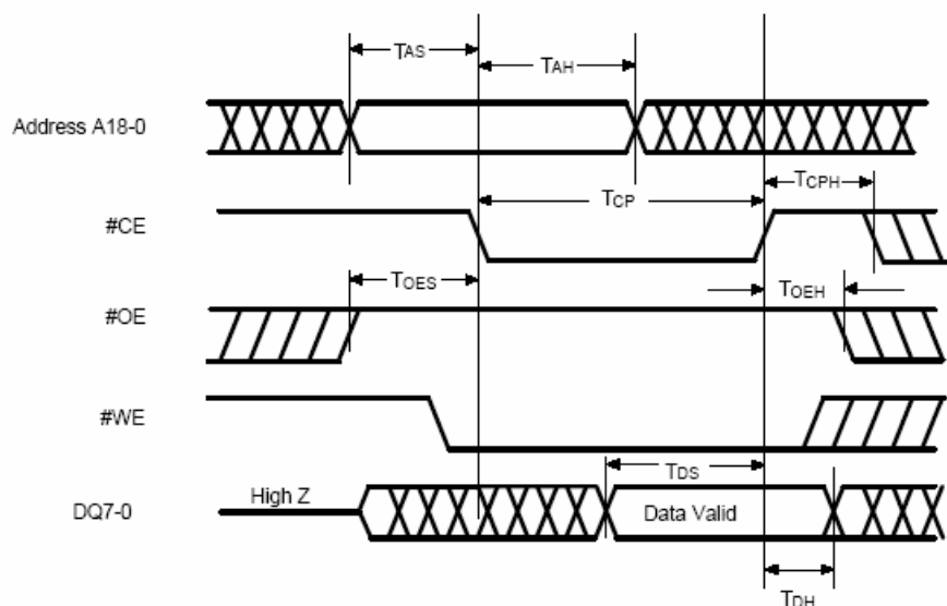
Figure 6-9. #CE Controlled Command Write Cycle Timing Diagram
