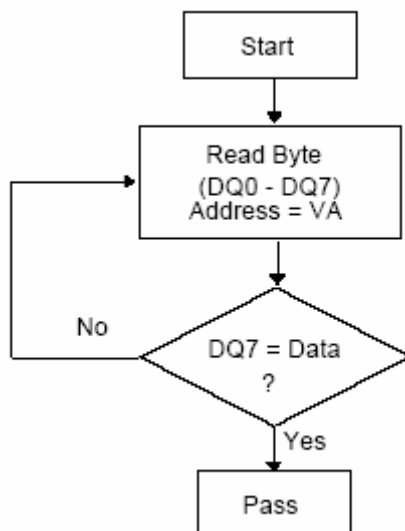
Figure 6-5.Embedded #Data Polling Algorithm State Diagram
