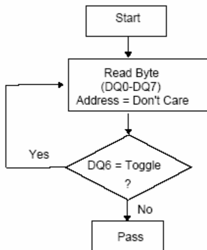
Figure 6-6.Embedded Toggle Bit Algorithm State Diagram
