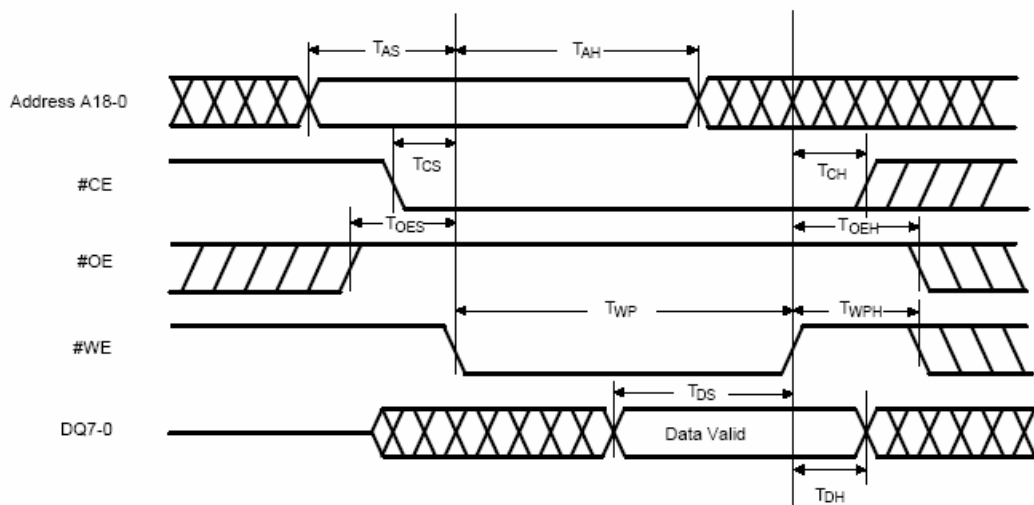
Figure 6-8. #WE Controlled Command Write Cycle Timing Diagram
