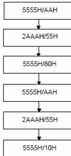
Figure 6-4.Embedded Erase Algorithm State Diagram
