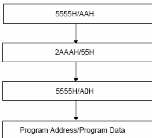
Figure 6-3.Embedded Programming Algorithm State Diagram
