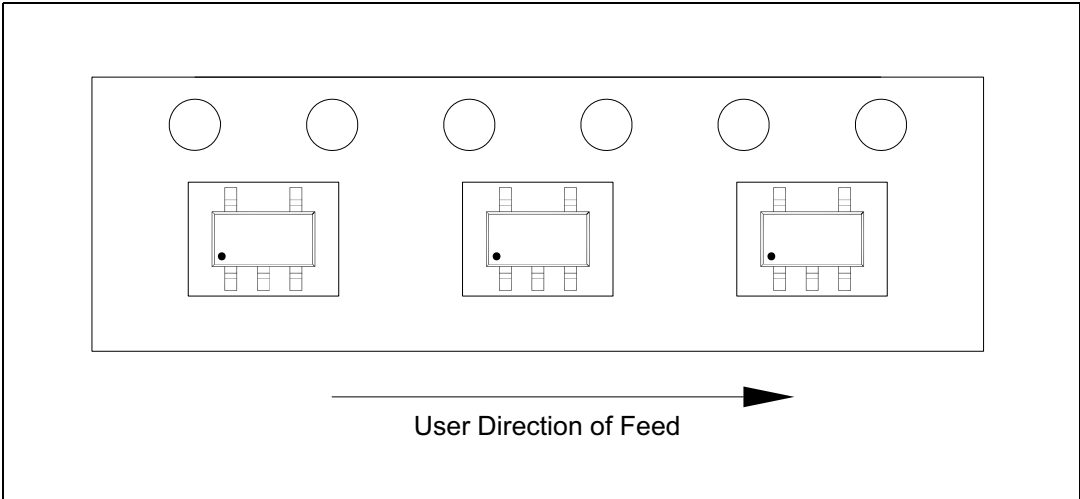
Figure 26. SOT23-5L oriented tape outline
