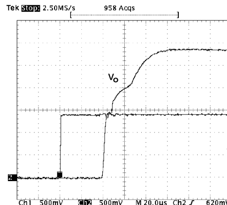
Figure 21. Startup
