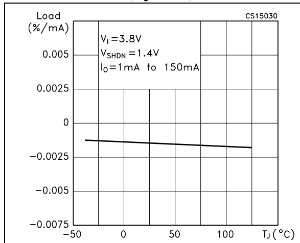
Figure 14. Load regulation vs. temperature ( V_0=3.3\text{ V} )
