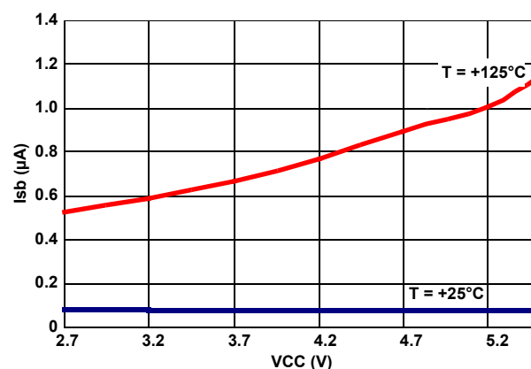
FIGURE 2. STANDBY I_{sb} vs V_{CC}
