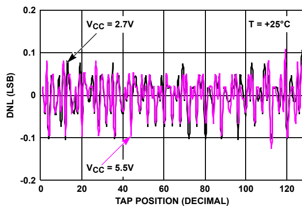
FIGURE 3. DNL vs TAP POSITION IN VOLTAGE DIVIDER MODE FOR 10k \Omega (W)
