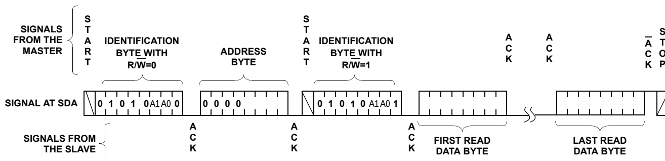
FIGURE 15. READ SEQUENCE
