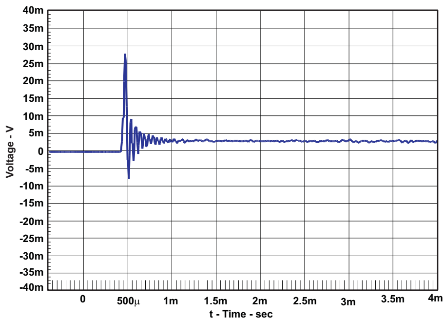
Figure 24. Pop/Click (PBTL)
