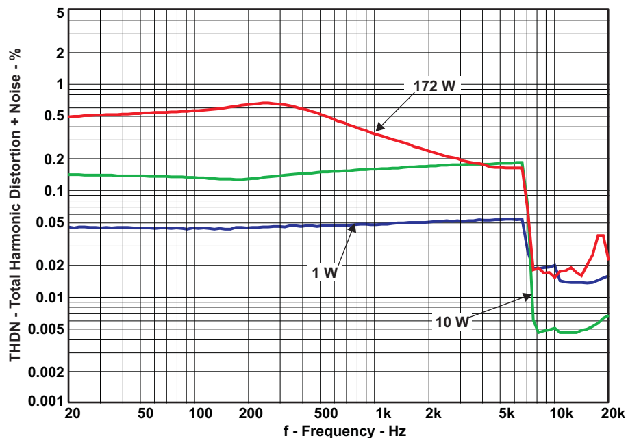
Figure 12. THD+N vs Frequency (PBTL –2 \Omega )
