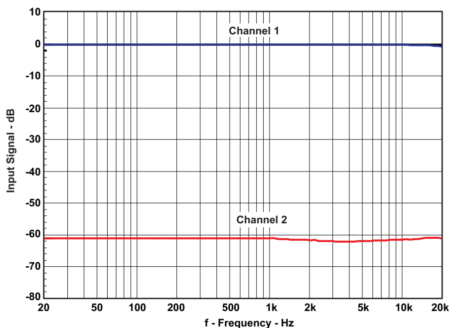
Figure 18. Channel Separation
