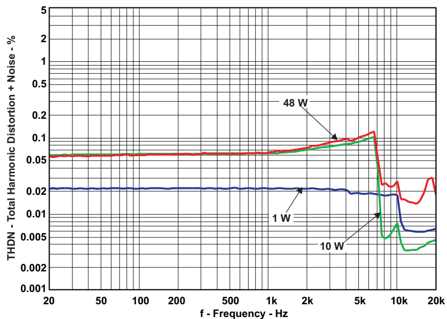
Figure 11. THD+N vs Frequency (BTL –8 \Omega )
