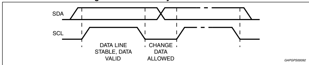
Figure 22. Data validity on the I 2 C bus
