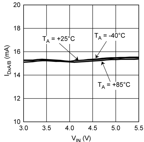
Diode Current vs Input Voltage
