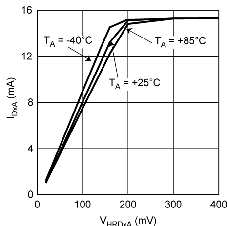
BankA Diode Current vs BankA Headroom Voltage
