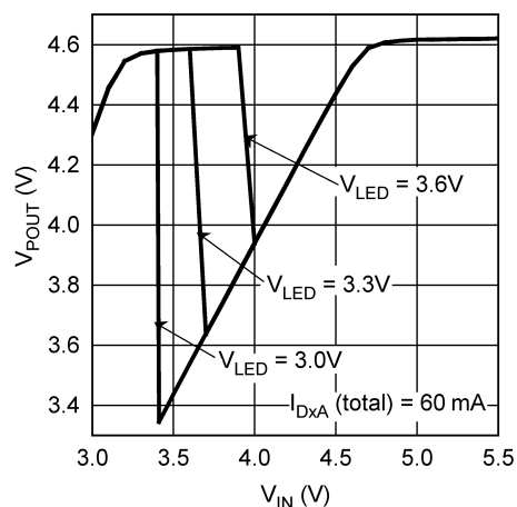
Charge Pump Output Voltage vs Input Voltage
