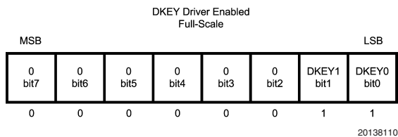
FIGURE 9. Internal Hex Address: B0h
