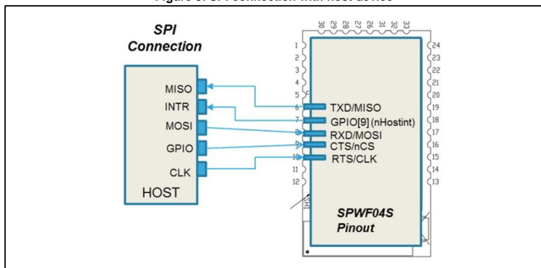
Figure 3: SPI connection with host device
