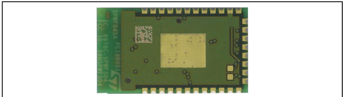
Figure 12: SPWF04SA bottom side
