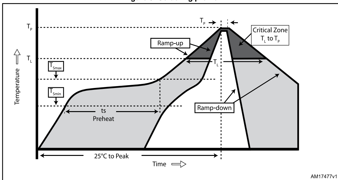
Figure 9: Soldering profile
