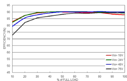
THN 30-4811WI Efficiency VS Output Current
