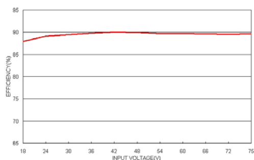
THN 30-4811WI Efficiency VS Input Voltage
