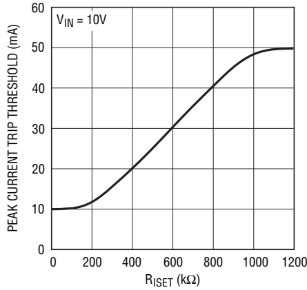
Peak Current Trip Threshold vs R_{\text{ISET}}
