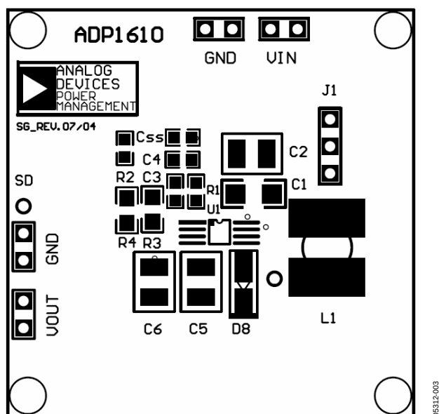
Figure 3. Top Silkscreen
