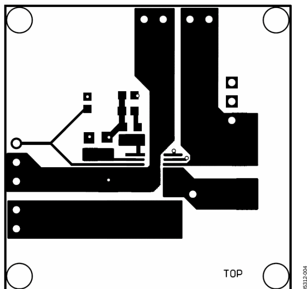
Figure 4. Top Layer
