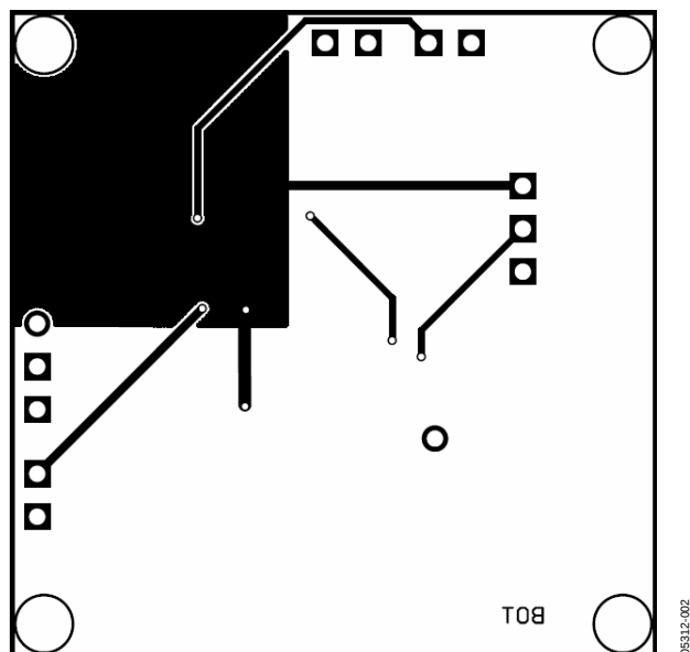
Figure 2. Bottom Layer
