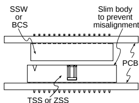
Board Stacking
