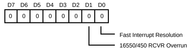
Figure 72. MIMIC Modification Register (Z180 MPU Write only, Address xxE9h)
