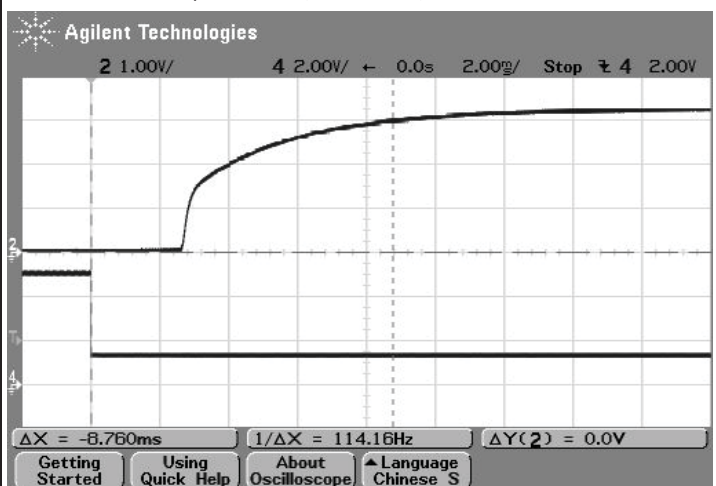
On/Off Enable Delay (Vin=48V, Vout=nom., Iout=25A, Cload=10uF, Ta=+25° C., ScopeBW=20Mhz, Trace 2=Vout, Trace 4=Enable.
