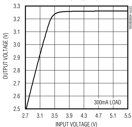
LD03 OUTPUT VOLTAGE vs. INPUT VOLTAGE
