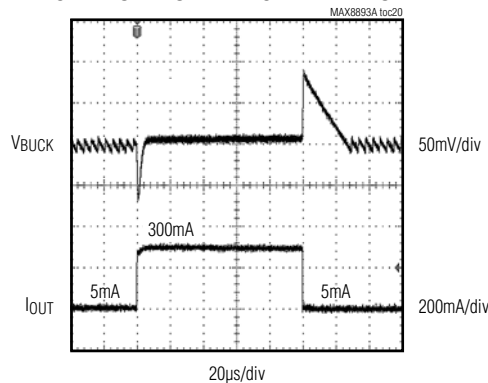
STEP-DOWN LOAD TRANSIENT WAVEFORM
