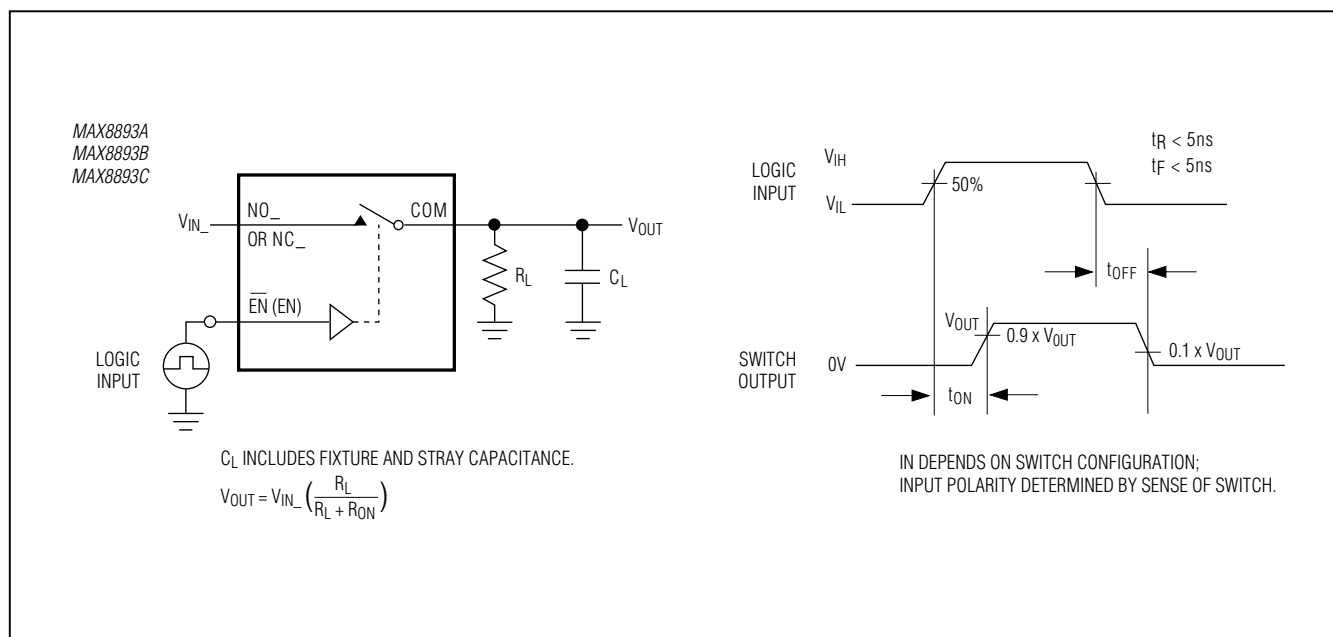
Figure 2. USB High-Speed Switch Switching Time
