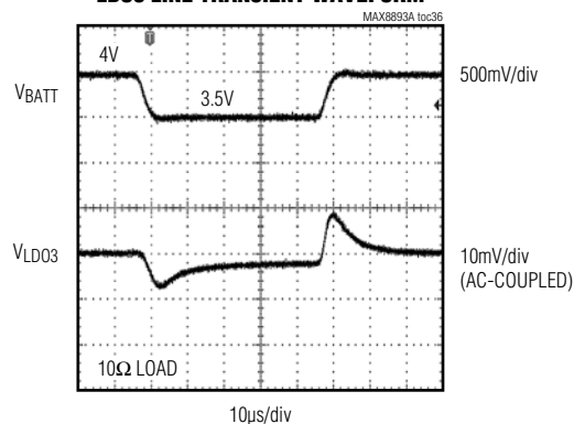
LD03 LINE TRANSIENT WAVEFORM
