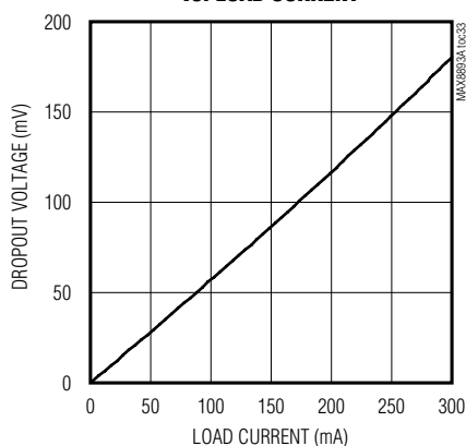
LD03 DROPOUT VOLTAGE vs. LOAD CURRENT
