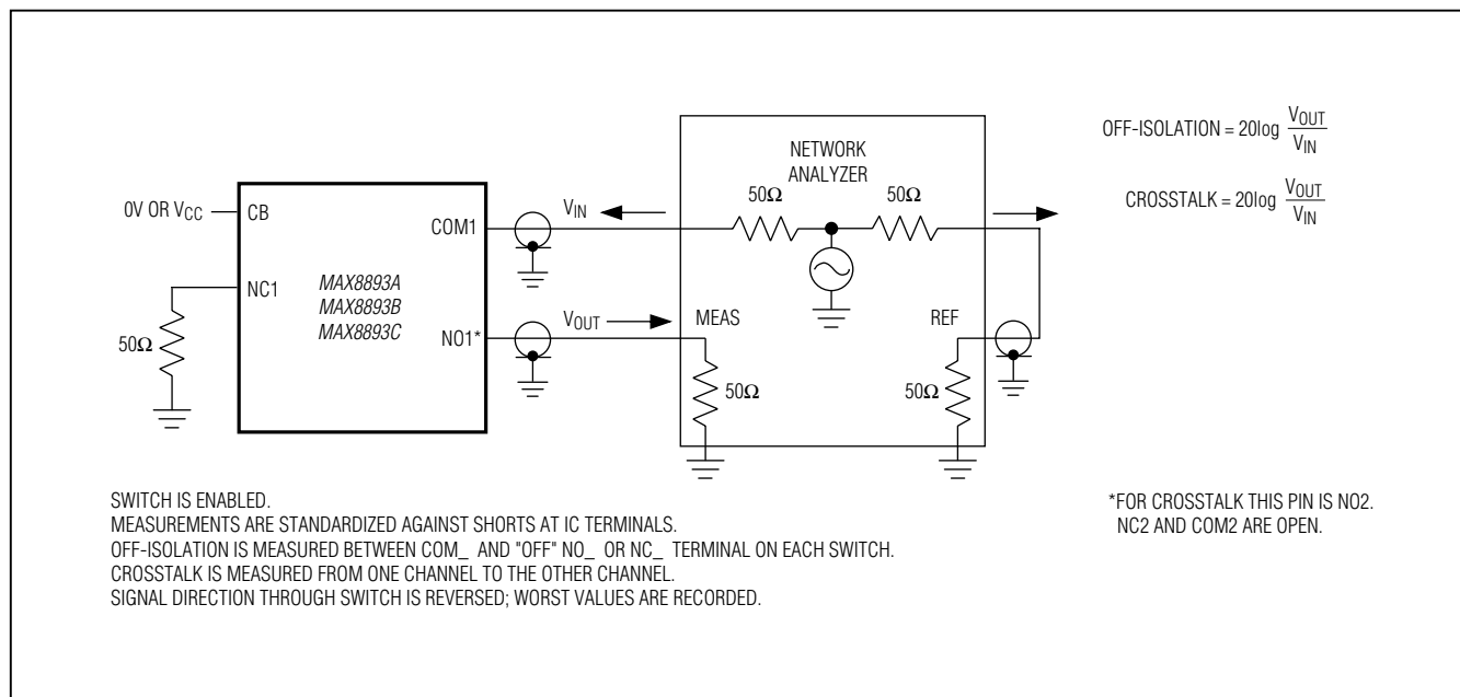
Figure 1. USB High-Speed Switch Off-Isolation and Crosstalk
