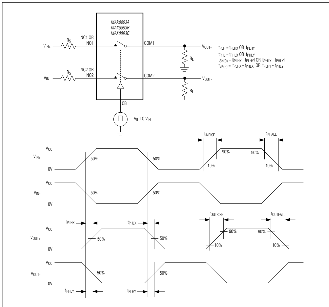
Figure 3. USB High-Speed Switch Output Signal Skew, Rise/Fall Time, Propagation Delay
