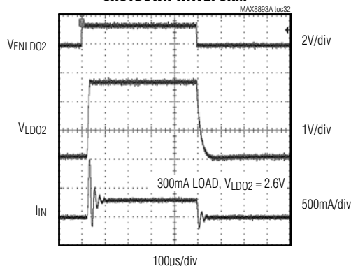
LD02 STARTUP AND SHUTDOWN WAVEFORM
