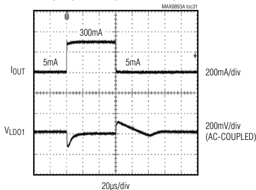
LD02 LOAD TRANSIENT WAVEFORM
