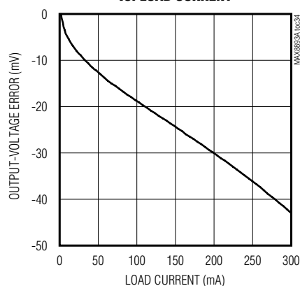
LD03 OUTPUT-VOLTAGE ERROR vs. LOAD CURRENT
