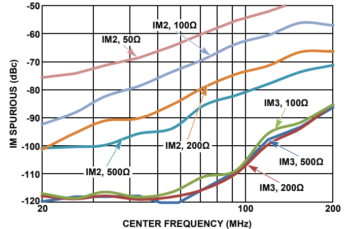
FIGURE 13. IM2 AND IM3 vs R_{LOAD}
