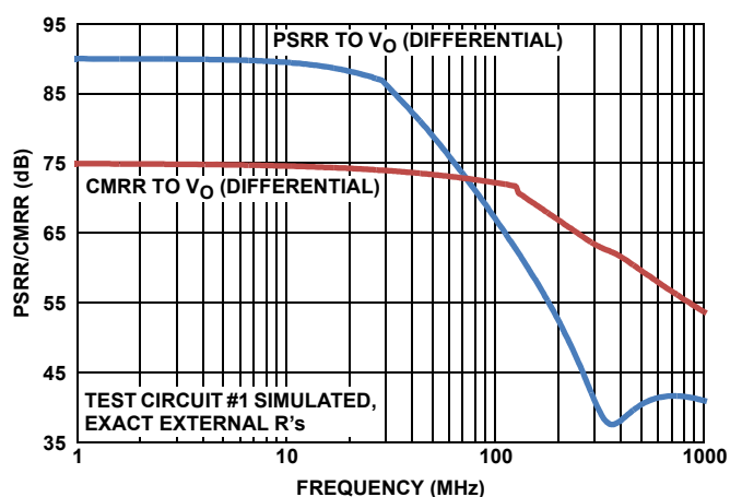
FIGURE 25. PSRR/CMRR TO DIFFERENTIAL V_0
