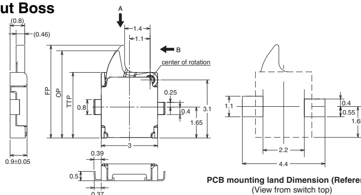
PCB mounting land Dimension (Reference) (View from switch top)
