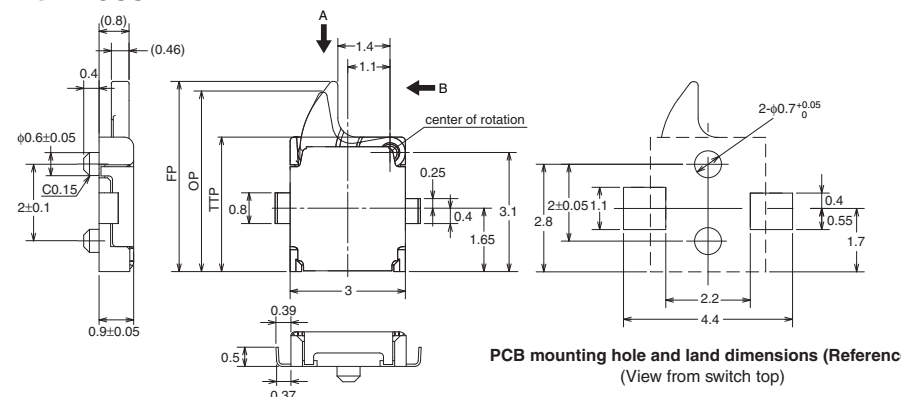
PCB mounting hole and land dimensions (Reference) (View from switch top)
