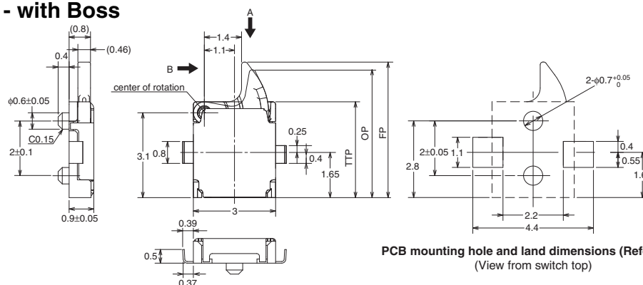
PCB mounting land Dimension (Reference) (View from switch top)
