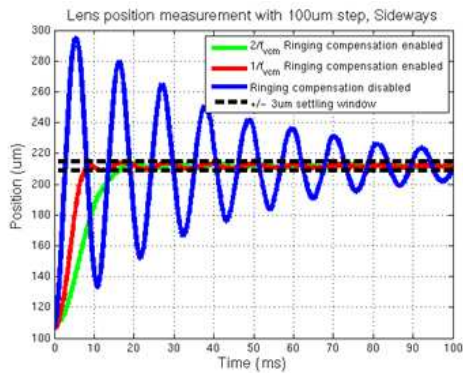
Figure 22. Lens Positions With and Without Ringing Compensation With 100-μm Step on the Lens Position
