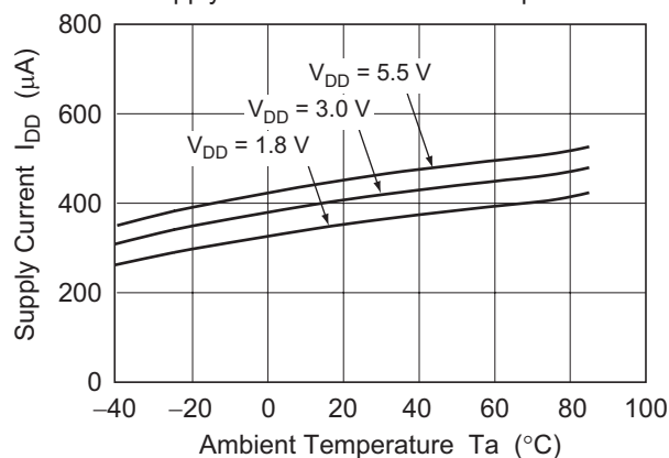
Figure 2-2. HA1630S05 Supply Current vs. Ambient Temperature
