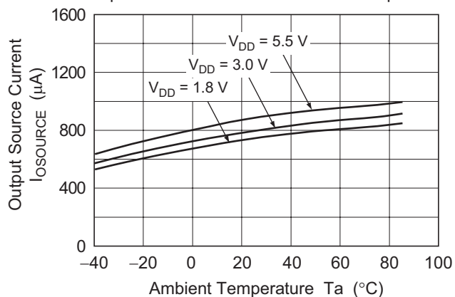
Figure 3-5. HA1630S06 Output Source Current vs. Ambient Temperature
