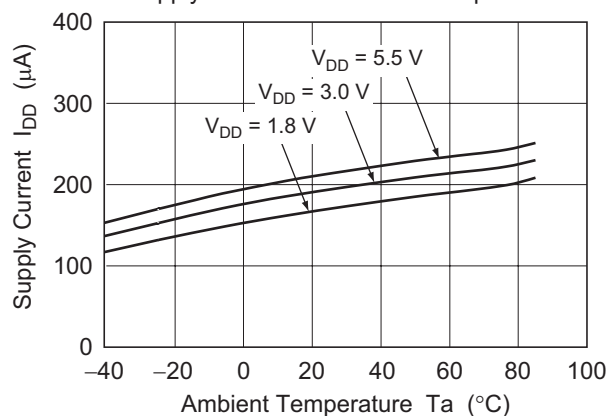
Figure 1-2. HA1630S04 Supply Current vs. Ambient Temperature
