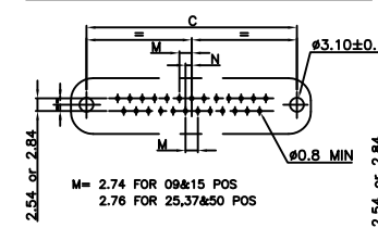
PCB DRILLING DETAIL - 09 TO 37 POS
