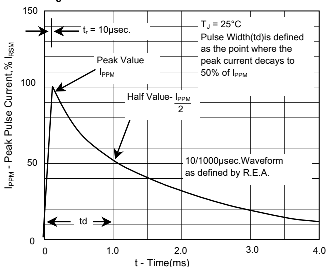
Fig. 3 - Pulse Waveform
