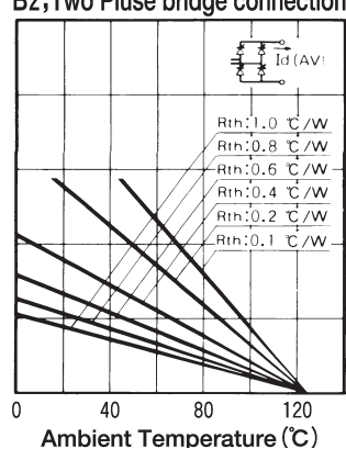
B2; Two Pulse bridge connection
