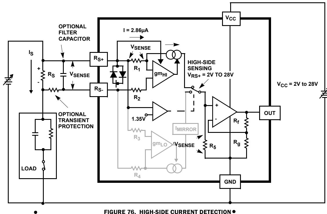
FIGURE 76. HIGH-SIDE CURRENT DETECTION •
