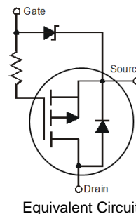
Equivalent Circuit
