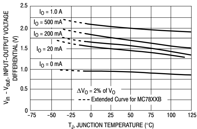
Figure 14. Input Output Differential as a Function of Junction Temperature (MC78XXC, AC, B)
