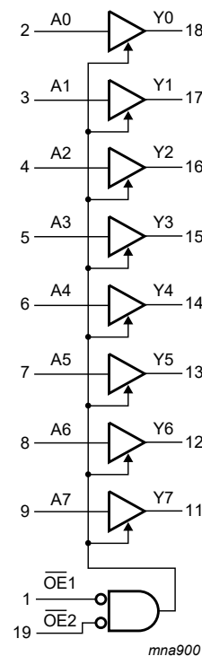
Fig. 2. Functional diagram
