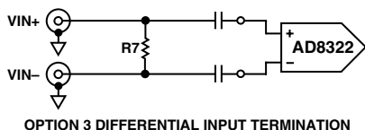
Figure 8. Differential Input Termination Options
