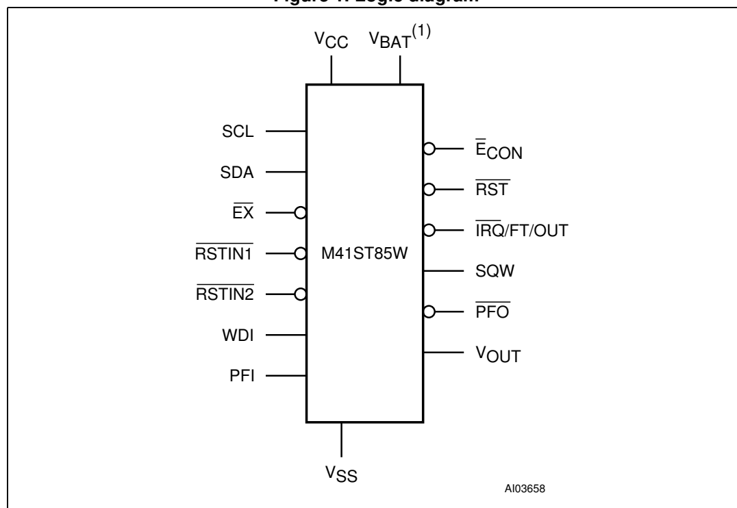
Figure 1. Logic diagram
