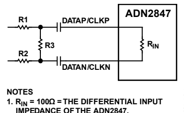
Figure 11. Attenuation Circuit
