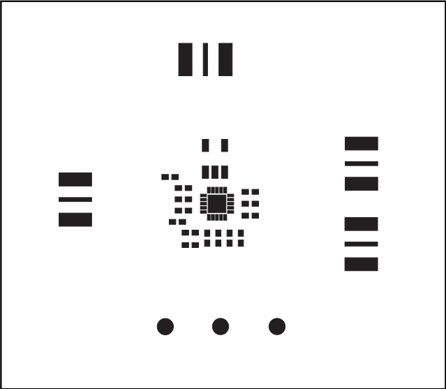
Figure 4. MAX2041 EV Kit PC Board Layout—Top Soldermask
