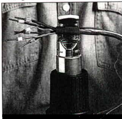
Shrink-fitting sleeves
