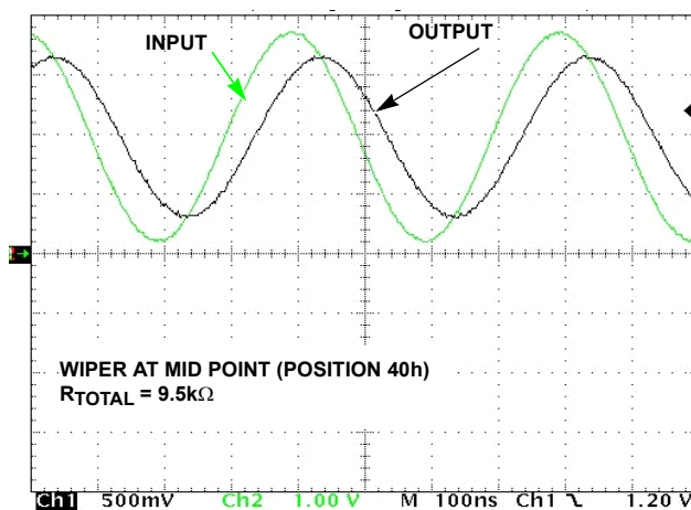
FIGURE 12. FREQUENCY RESPONSE (2.6MHz)
