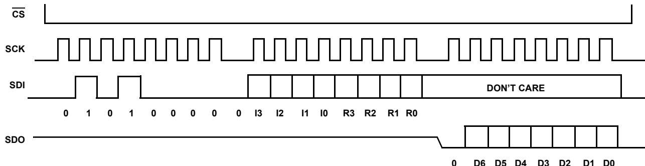
FIGURE 17. THREE BYTE READ SEQUENCE
