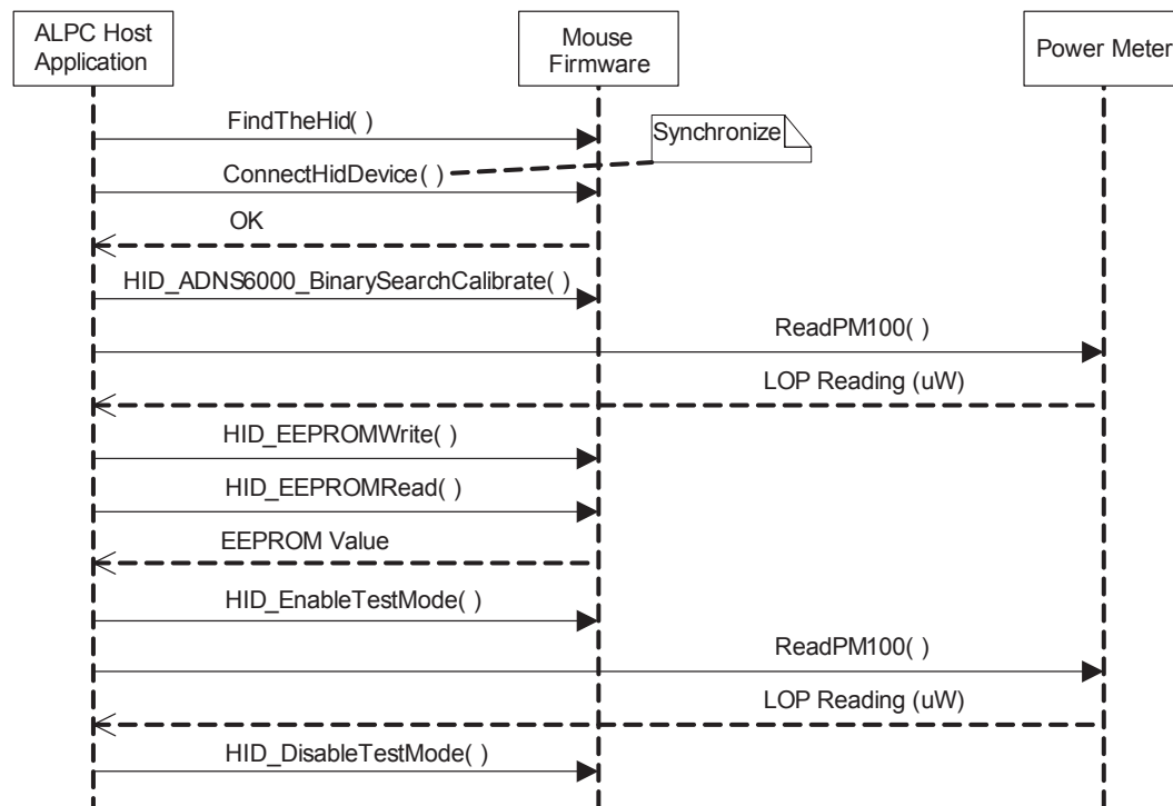
Figure 2.0 PC host application laser output power calibration flow sequence diagram
