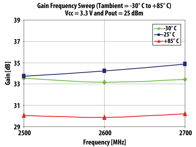
Figure 8. Gain Frequency Sweep at V_{cc} = 3.3\text{ V} and P_{out} = 25\text{ dBm} over T_{ambient}
