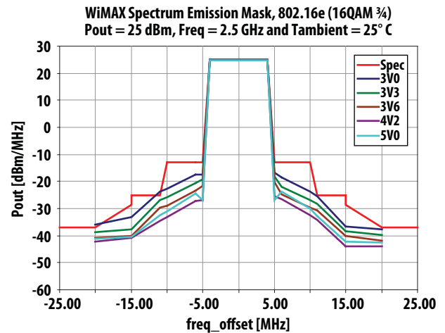
Figure 20. SEM at V_{cc} = 3.3 V, 25^{\circ}\text{C} and 2.5 GHz over V_{cc} (2dB Post-PA loss assumed)
