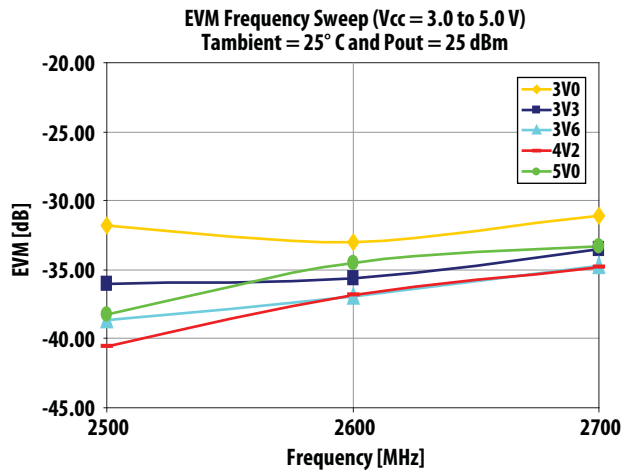
Figure 1. EVM Frequency Sweep at 25^{\circ}\text{C} and P_{out} = 25 dBm over V_{cc}
