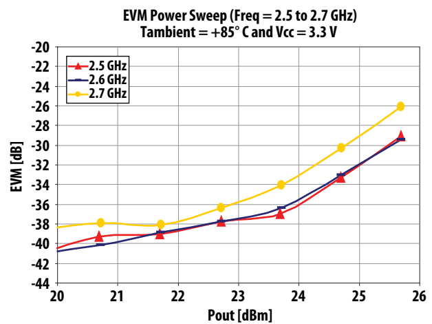
Figure 6. EVM Power Sweep at V_{cc} = 3.3 V and +85^{\circ}\text{C} over Frequency
