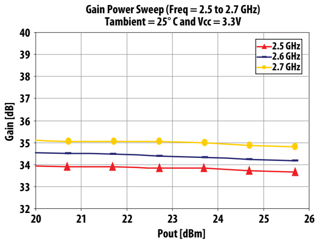
Figure 9. Gain Power Sweep at V_{cc} = 3.3\text{ V} and 25^\circ\text{C} over P_{out}
