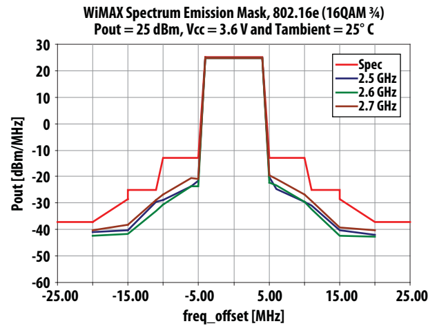
Figure 18. SEM Frequency Sweep at V_{cc} = 3.6 V and 25^{\circ}\text{C} (2dB Post-PA loss assumed)
