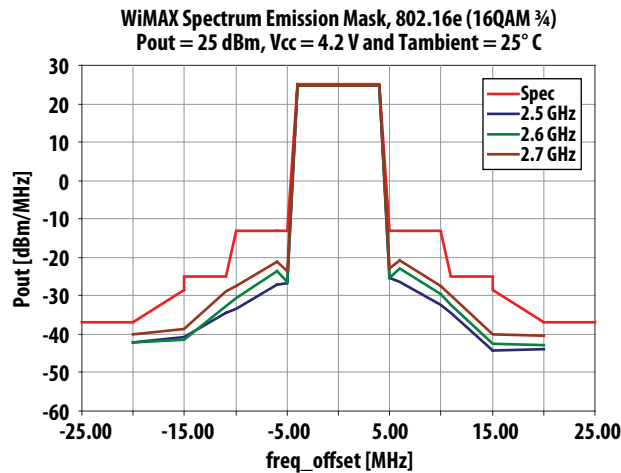
Figure 19. SEM Frequency Sweep at V_{cc} = 4.2 V and 25^{\circ}\text{C} (2 dB Post-PA loss assumed)
