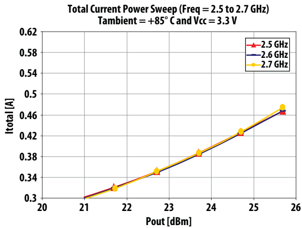
Figure 16. Total Current Power Sweep at 3.3 V and +85^{\circ}\text{C} over Frequency
