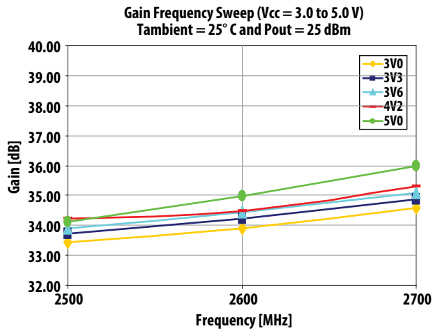
Figure 7. Gain Frequency Sweep at 25^\circ\text{C} and P_{out} = 25\text{ dBm} over V_{cc}
