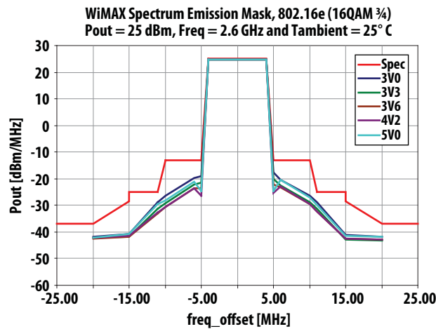
Figure 21. SEM at V_{cc} = 3.3 V, 25^{\circ}\text{C} and 2.6 GHz over V_{cc} (2 dB Post-PA loss assumed)
