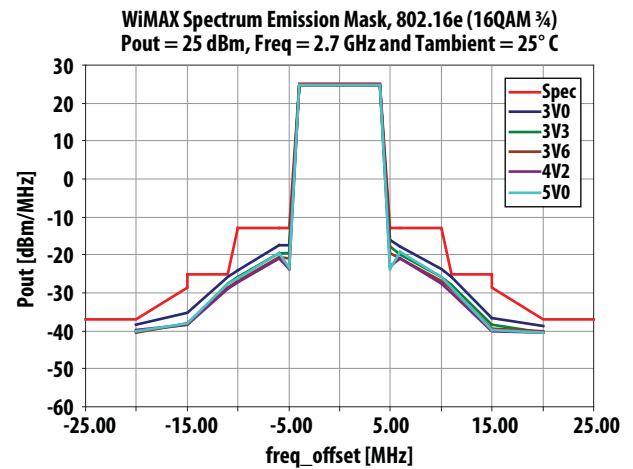
Figure 22. SEM at V_{cc} = 3.3 V, 25^{\circ}\text{C} and 2.7 GHz over V_{cc} (2dB Post-PA loss assumed)
