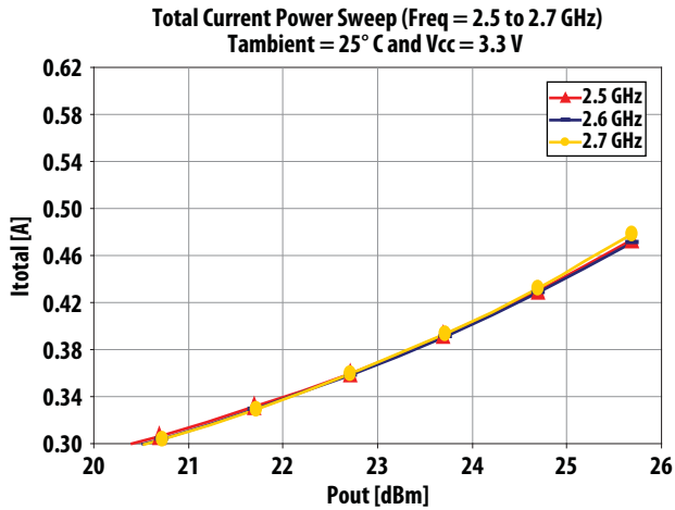
Figure 14. Total Current Power Sweep at 3.3 V and 25^{\circ}\text{C} over Frequency
