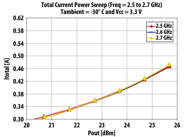
Figure 15. Total Current Power Sweep at 3.3 V and -30^{\circ}\text{C} over Frequency
