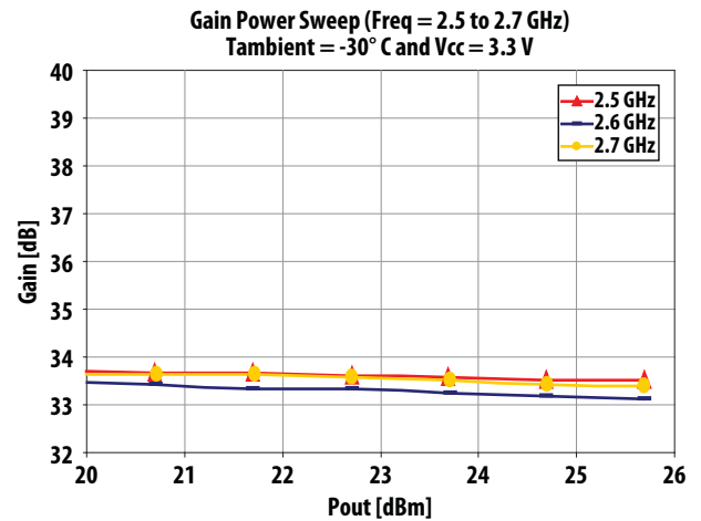
Figure 10. Gain Power Sweep at V_{cc} = 3.3\text{ V} and -30^\circ\text{C} over P_{out}
