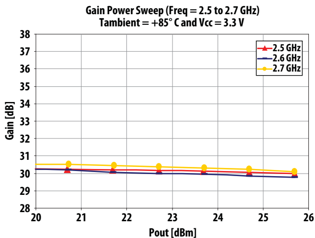
Figure 11. Gain Power Sweep at V_{cc} = 3.3\text{ V} and +85^\circ\text{C} over P_{out}
