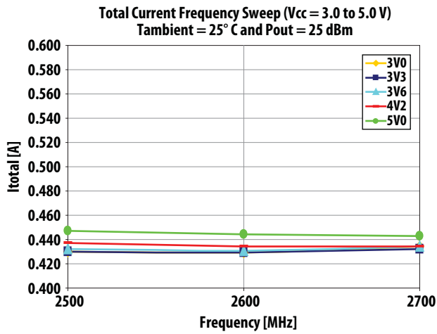
Figure 12. Total Current Frequency Sweep at 25^{\circ}\text{C} and P_{out} = 25 dBm over V_{cc}
