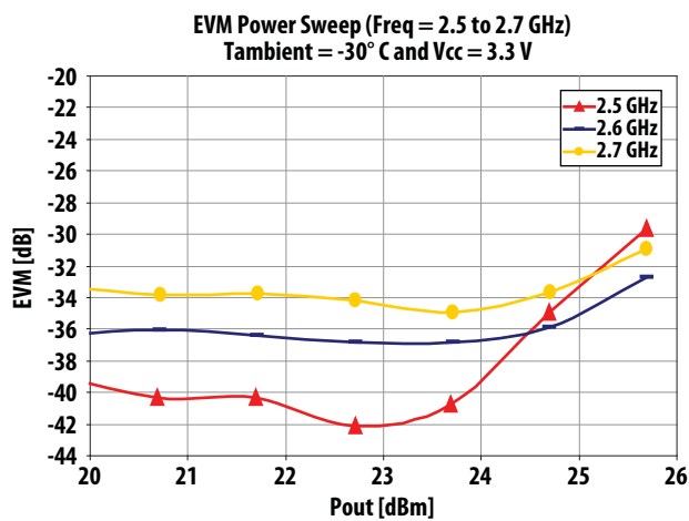
Figure 5. EVM Power Sweep at V_{cc} = 3.3 V and -30^{\circ}\text{C} over Frequency
