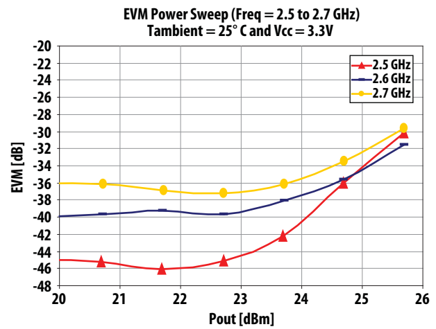
Figure 4. EVM Power Sweep at V_{cc} = 3.3 V and 25^{\circ}\text{C} over Frequency
