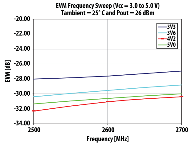
Figure 2. EVM Frequency Sweep at 25^{\circ}\text{C} and P_{out} = 26 dBm over V_{cc}
