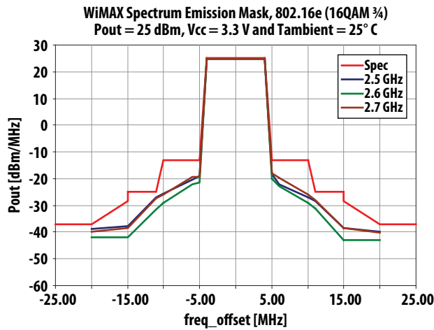
Figure 17. SEM Frequency Sweep at V_{cc} = 3.3 V and 25^{\circ}\text{C} (2 dB Post-PA loss assumed)
