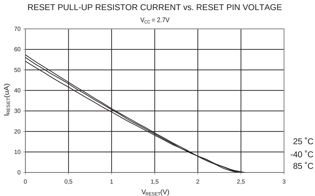
Figure 20-17. Reset Pull-up Resistor Current vs. Reset Pin Voltage ( V_{CC} = 2.7V )
