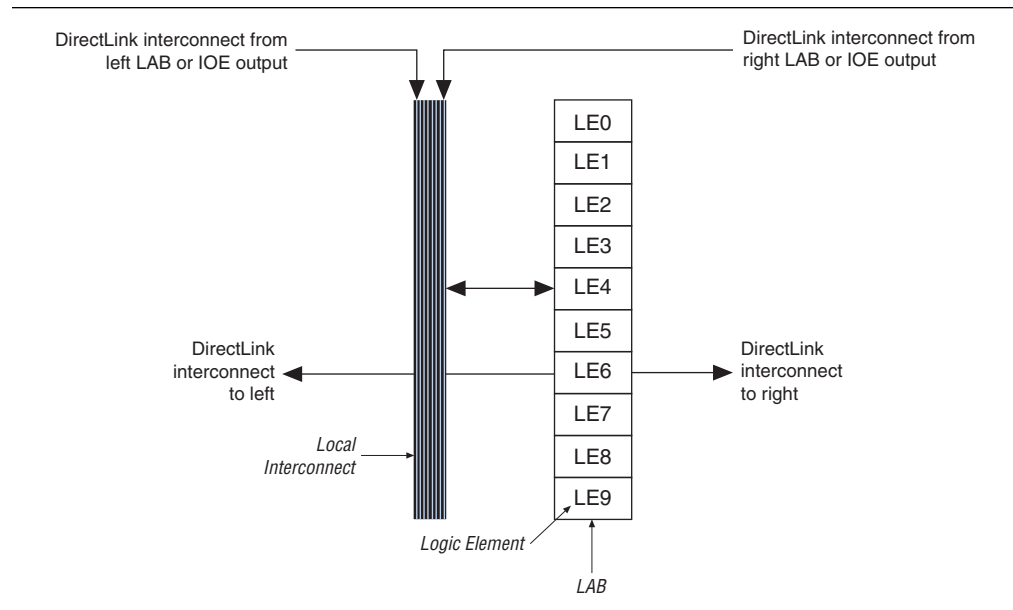
Figure 2-4. DirectLink Connection
