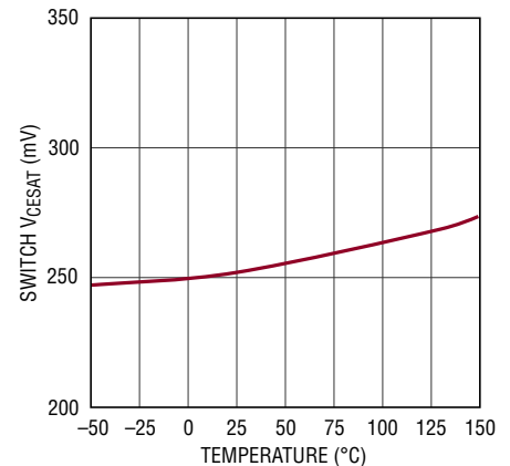
Switch V_{CESAT} ( I_{SW} = 500\text{mA} ) vs Temperature
