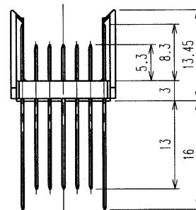
<Long pin>
