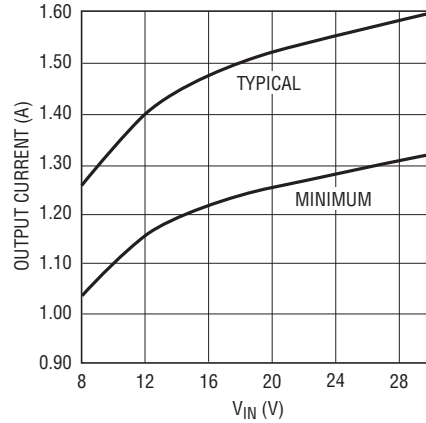
Maximum Load Current, V_{\text{OUT}} = 5\text{V} , L = 33\mu\text{H}
