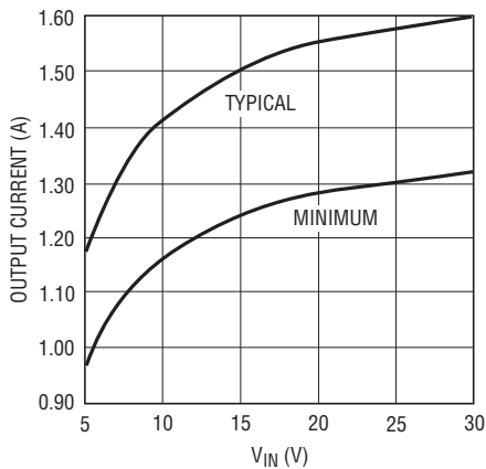
Maximum Load Current, V_{\text{OUT}} = 3.3\text{V} , L = 10\mu\text{H}
