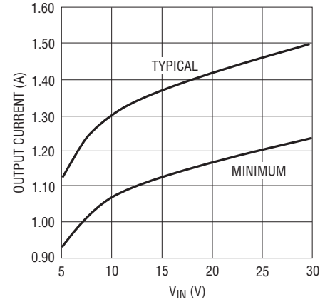
Maximum Load Current, V_{\text{OUT}} = 3.3\text{V} , L = 4.7\mu\text{H}
