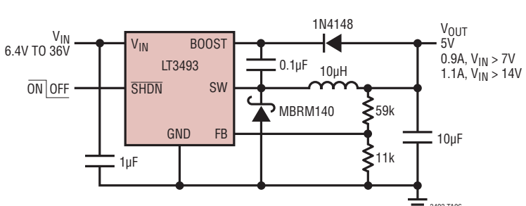
5V Step-Down Converter
