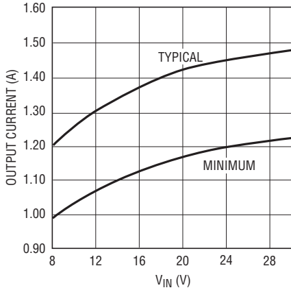
Maximum Load Current, V_{\text{OUT}} = 5\text{V} , L = 8.2\mu\text{H}
